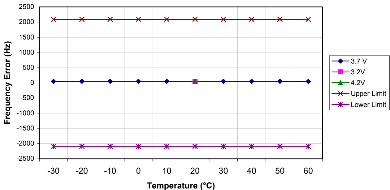
OVFKWC-KX21-2X0 AMPS 800 MHz Transmit RF Carrier Stability Over Temperature and Voltage
