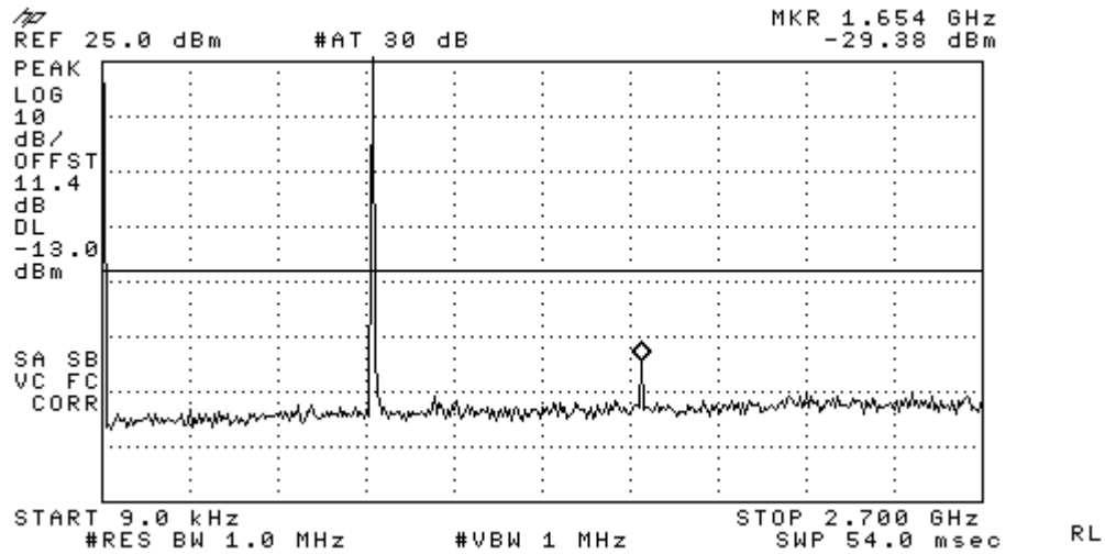
Figure 8-2a AMPS – Conducted Spurious Emission (CH 991)
