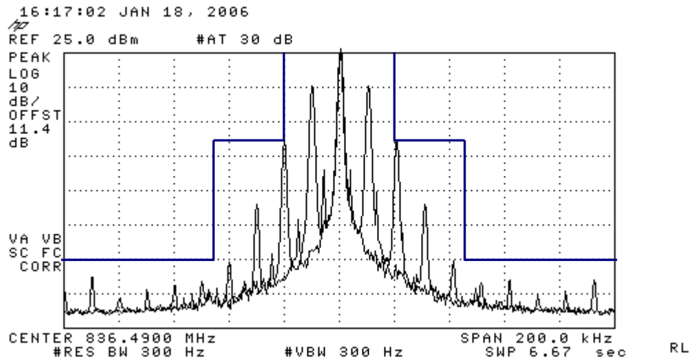
Figure 7-4 AMPS ST
