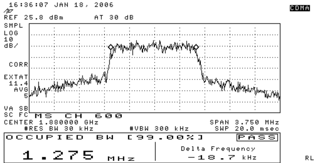
Figure 7-9 CDMA 1900 @ CH 600
