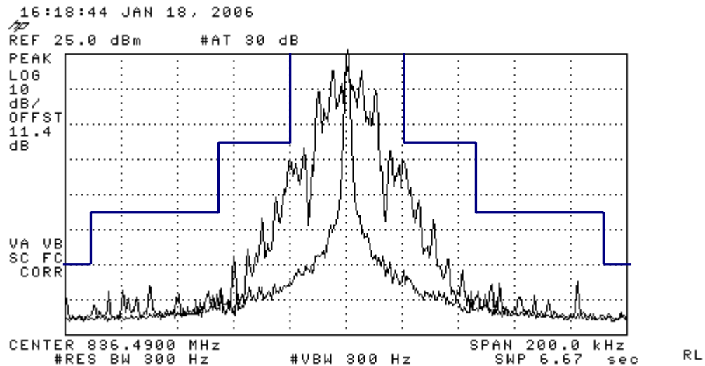
Figure 7-7 AMPS WIDEBAND
