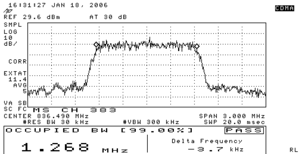
Figure 7-8 CDMA 800 @ CH 383
