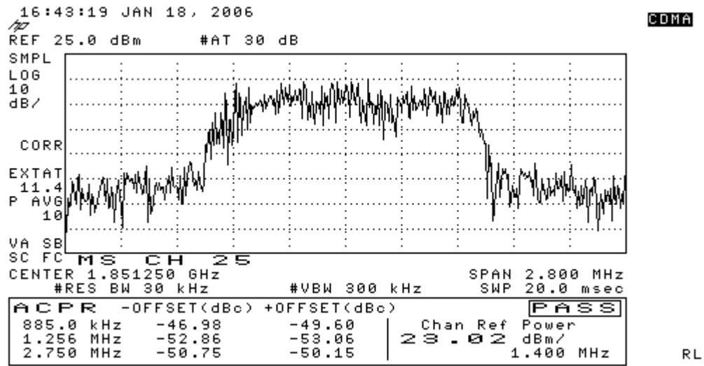
Figure 7-10 CDMA 1900 Lower Band Edge
