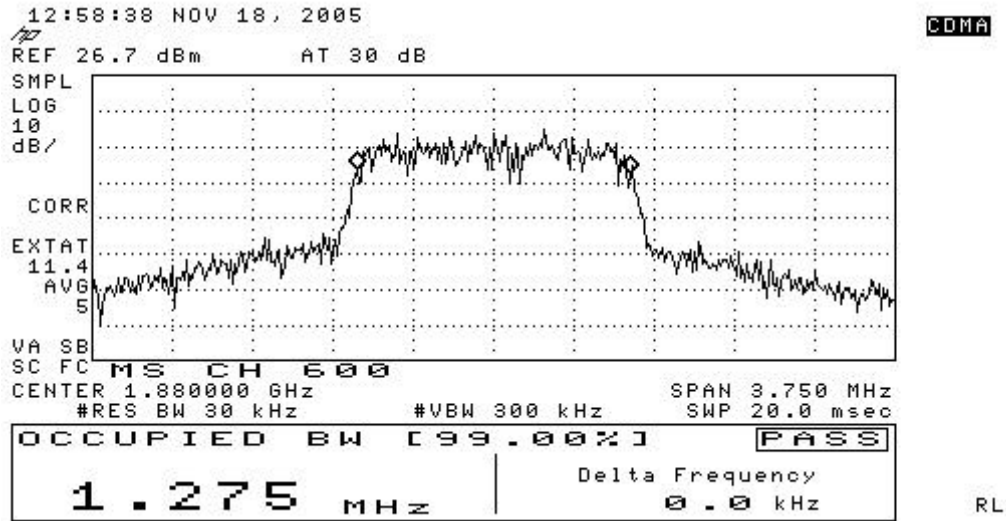
Figure 7-9 CDMA 1900 @ CH 600
