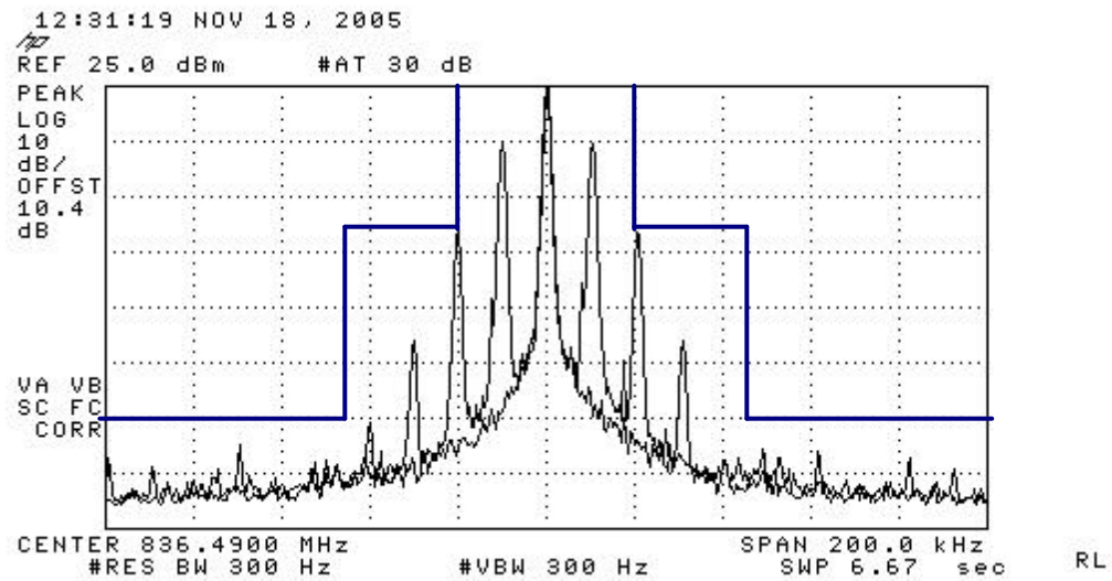
Figure 7-4 AMPS ST
