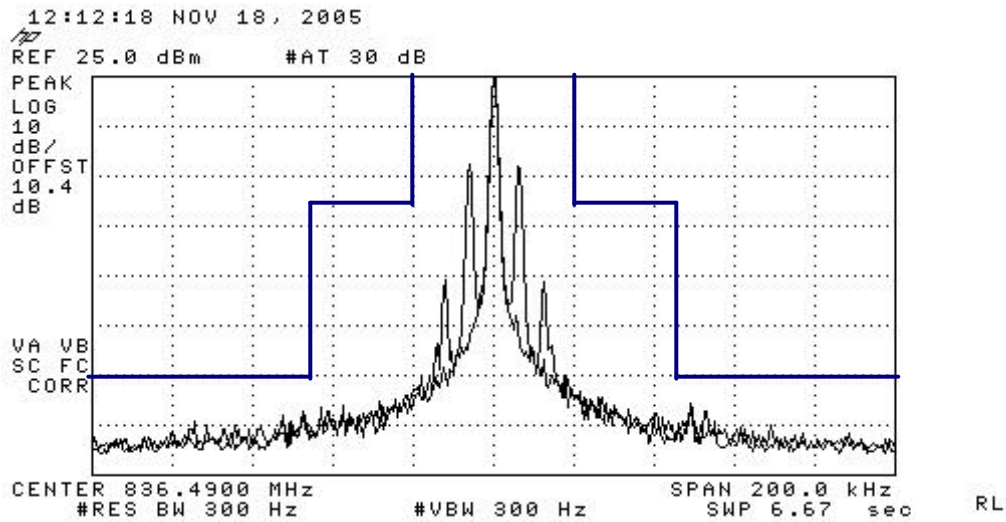
Figure 7-2 AMPS SAT
