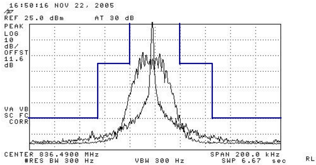
Figure 7-3 AMPS Voice + SAT
