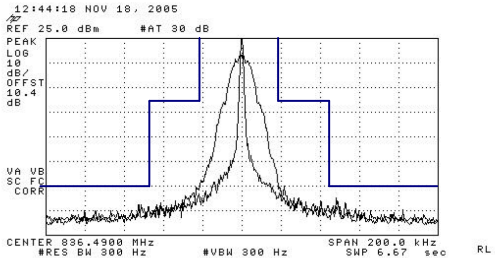
Figure 7-6 SAT + DTMF_9
