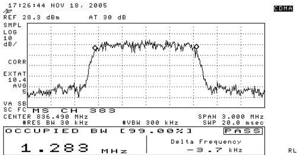
Figure 7-8 CDMA 800 @ CH 383
