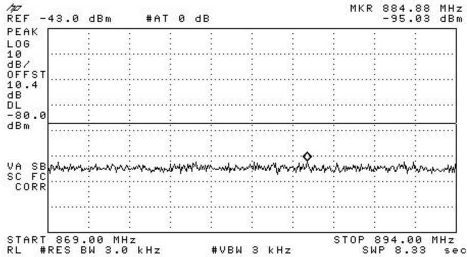
Figure 8-5 AMPS - Emissions in base station frequency range (CH 799)
