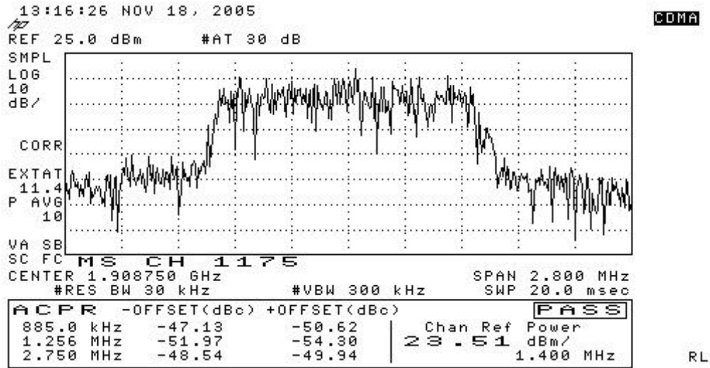
Figure 7-11 CDMA 1900 Upper Band Edge
