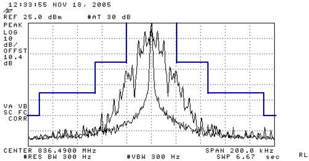
Figure 7-7 AMPS WIDEBAND
