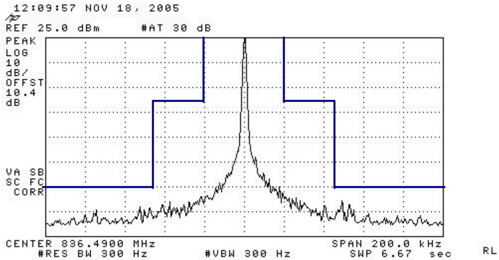
Figure 7-1 AMPS Unmodulated Signal
