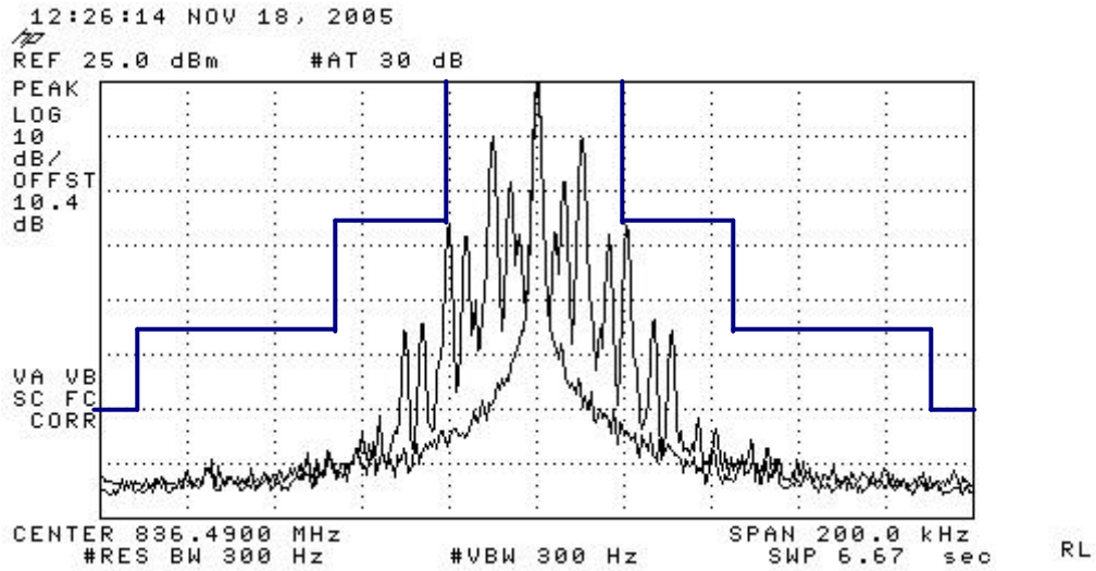
Figure 7-5 AMPS ST + SAT
