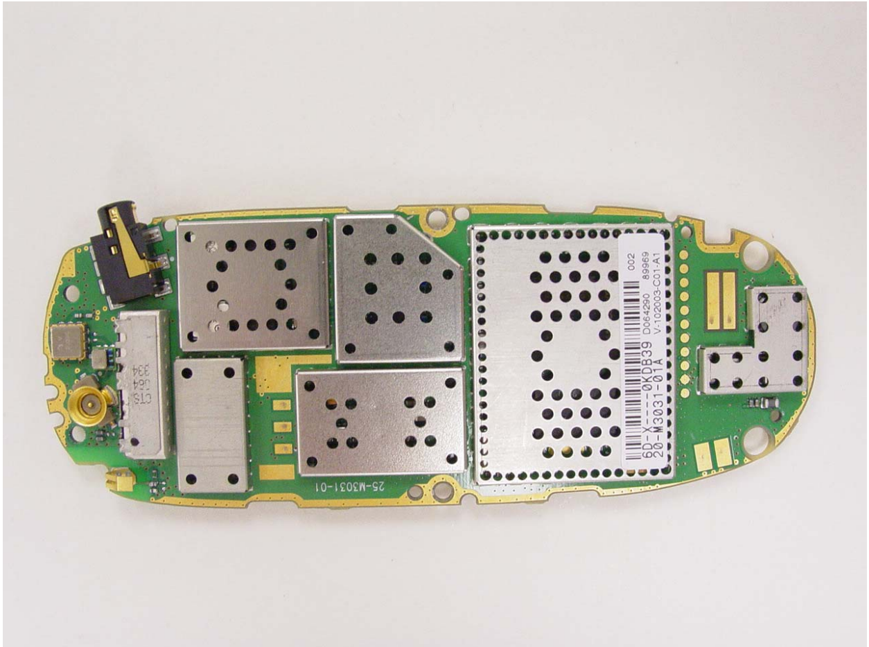
Main PCB_B
