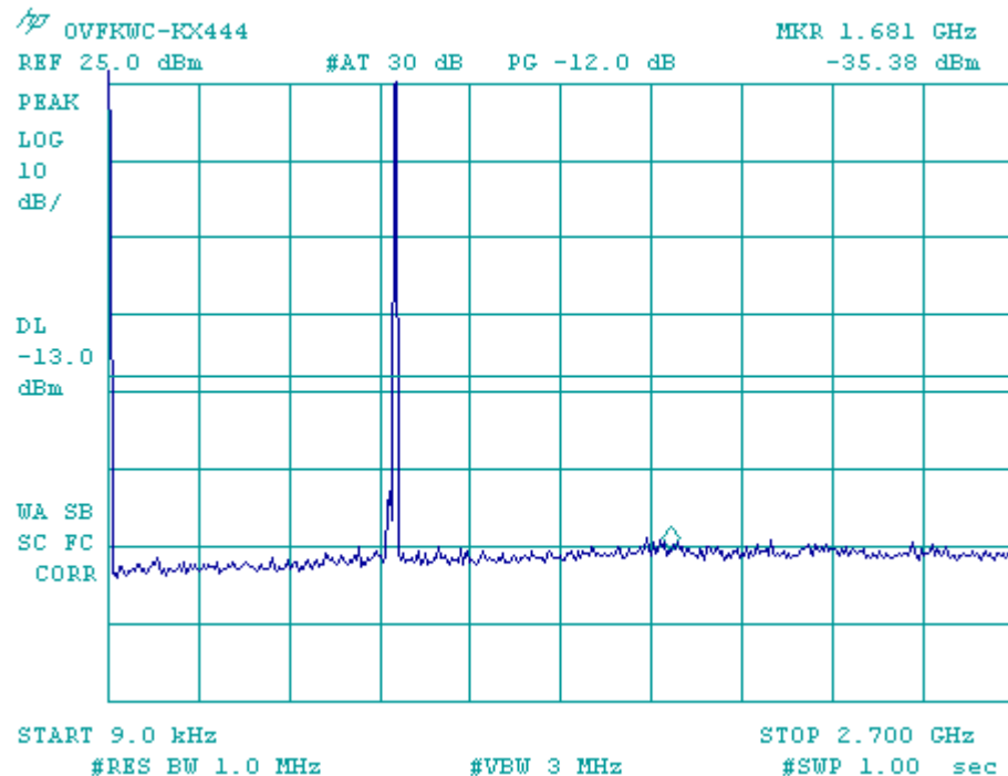
Figure 9-12a CDMA 800 – Conducted Spurious Emission (CH 777)
