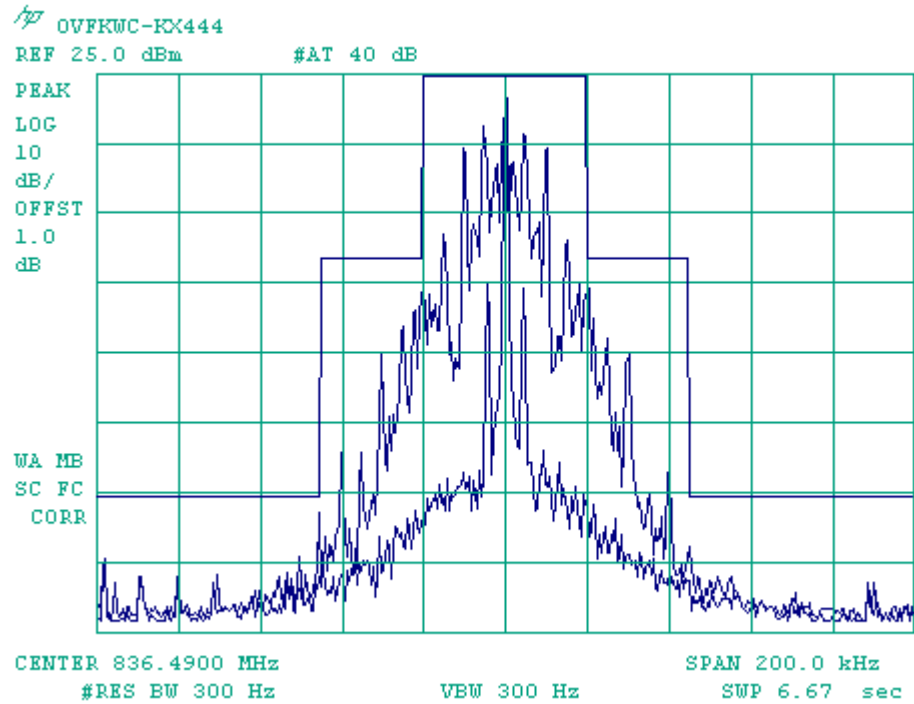
Figure 8-7 AMPS WIDEBAND
