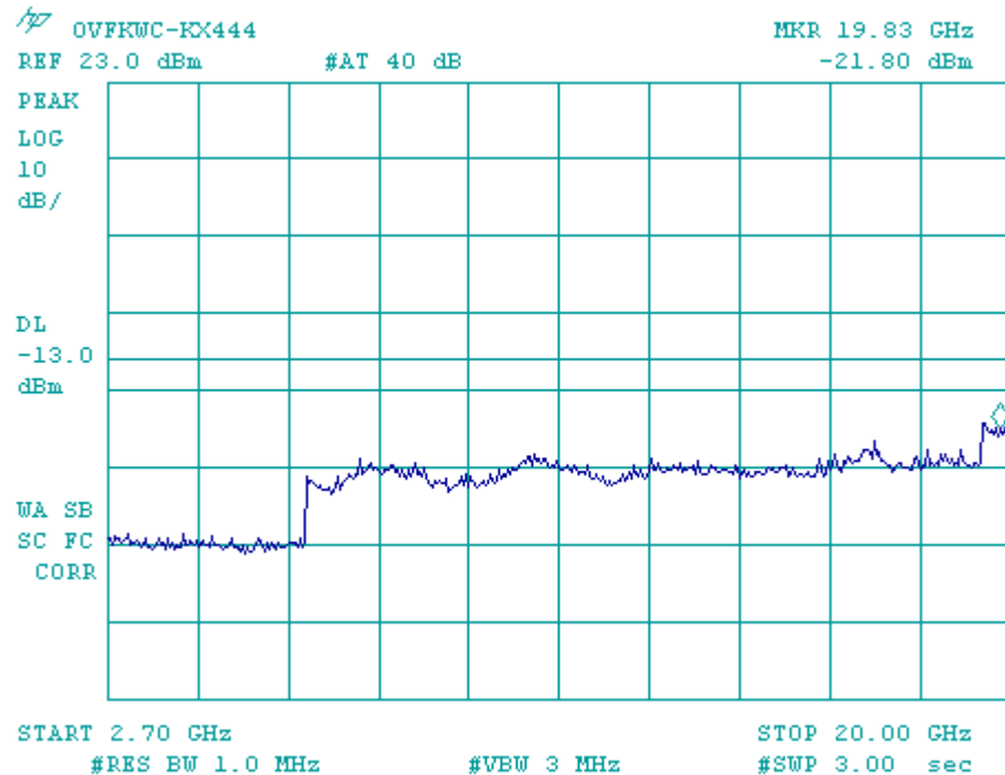
Figure 9-14b CDMA 1900 - Conducted Spurious Emission (CH 600)
