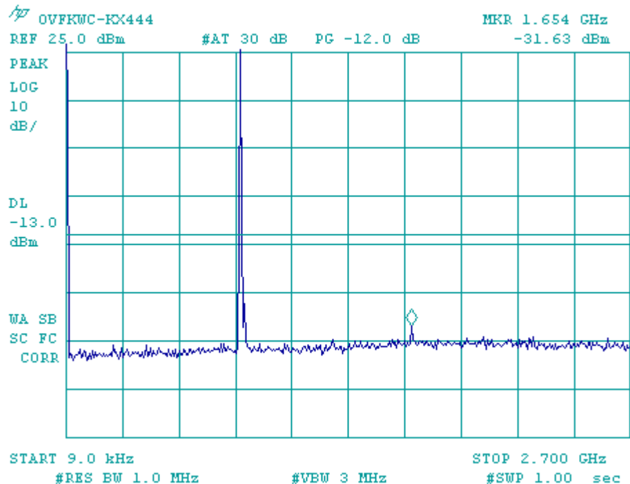
Figure 9-8a CDMA 800 – Conducted Spurious Emission (CH 1013)
