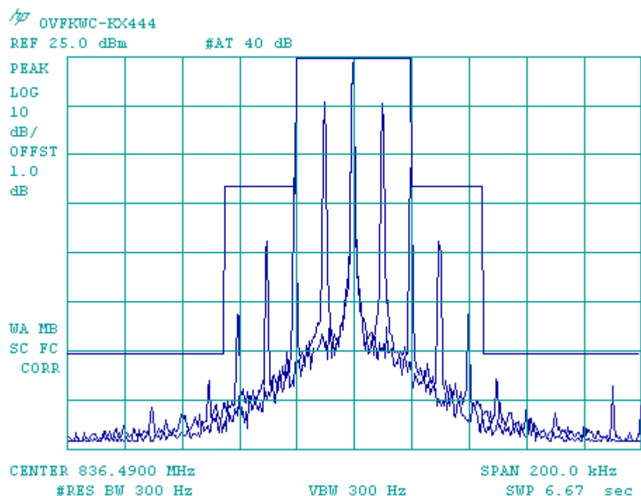
Figure 8-4 AMPS ST
