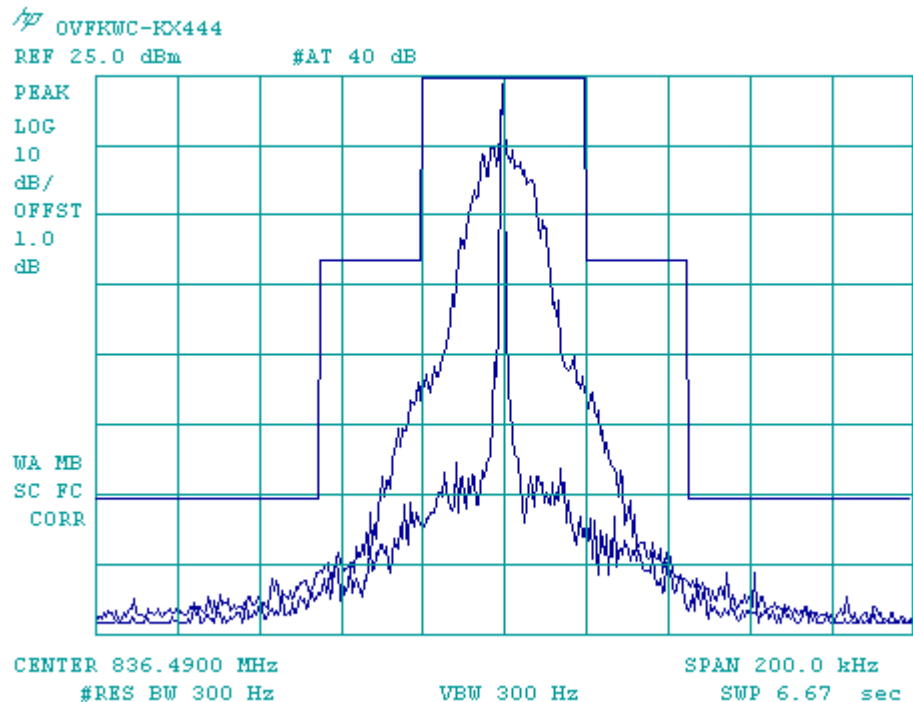
Figure 8-1 AMPS Voice
