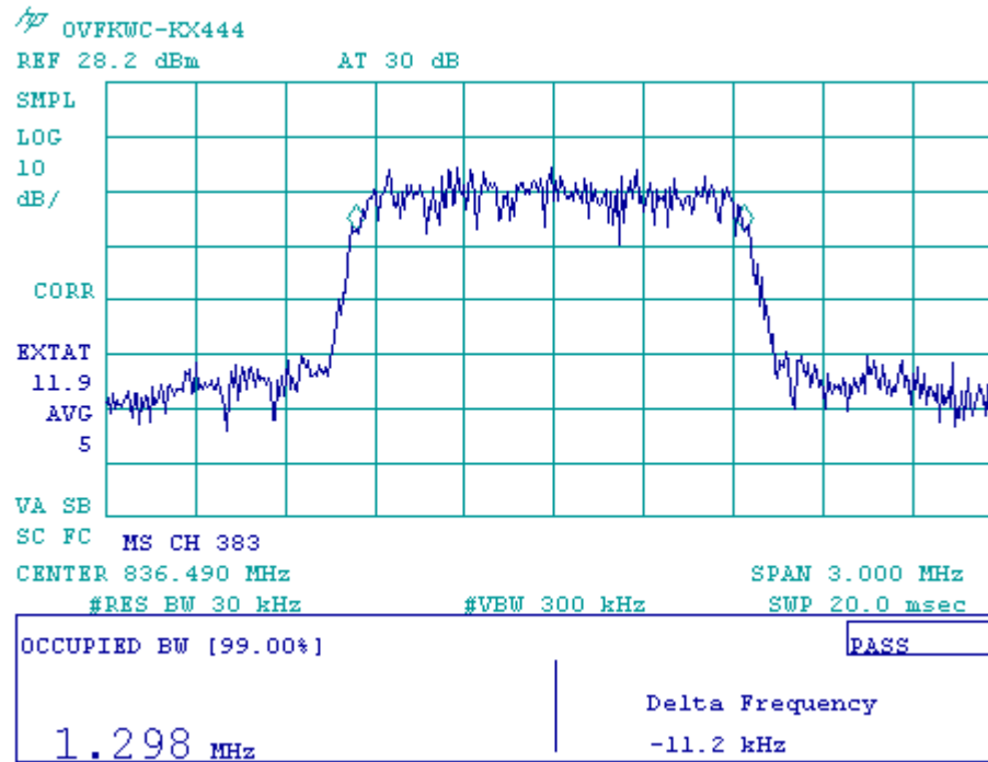
Figure 8-9c CDMA 800 1X at RC3 (F/R-FCH)
