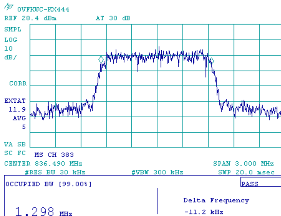
Figure 8-10c CDMA 800 1X at RC3 (F/R-FCH + F/R-SCH)
