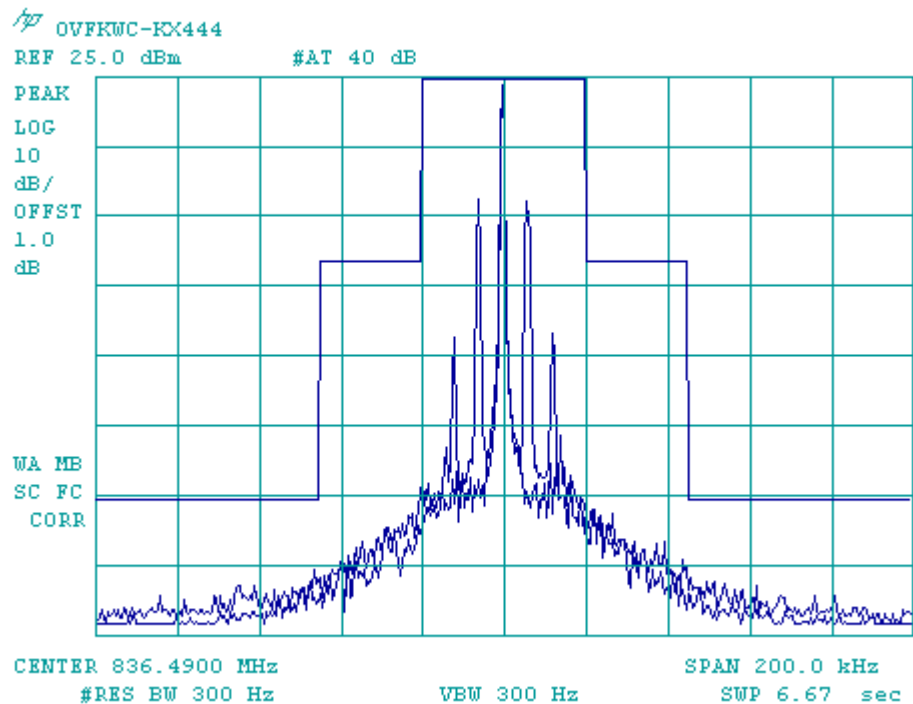
Figure 8-2 AMPS SAT
