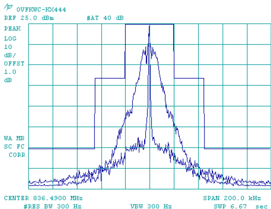
Figure 8-6 SAT + DTMF_9
