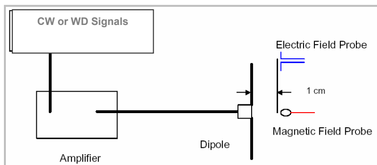
Figure 6 - Dipole Calibration
