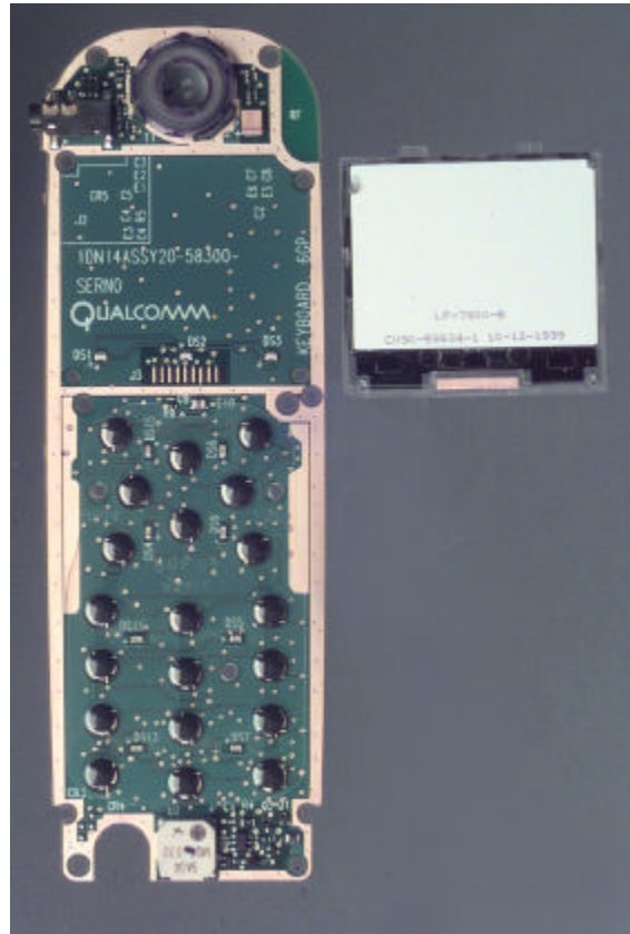
Key Board Front with LCD off
