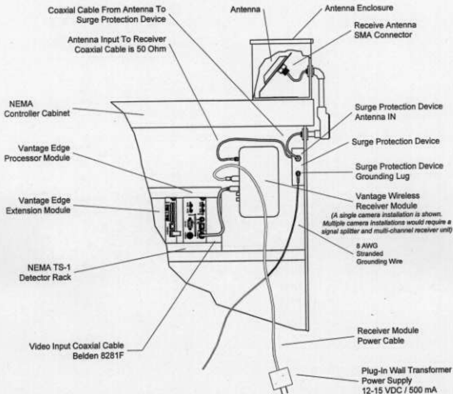
Optional Cabinet Top Mount Configuration (Shown)
