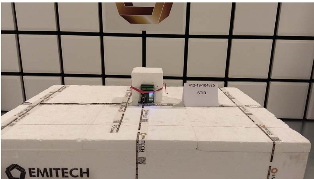
TEST SETUP PHOTO(S) RADIATED EMISSIONS POSITION 3
