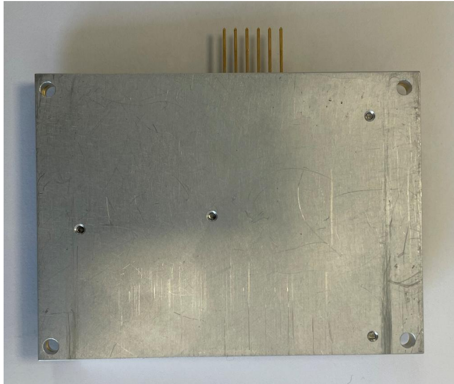
MUF electronic board with CEM shielding – Bottom side
