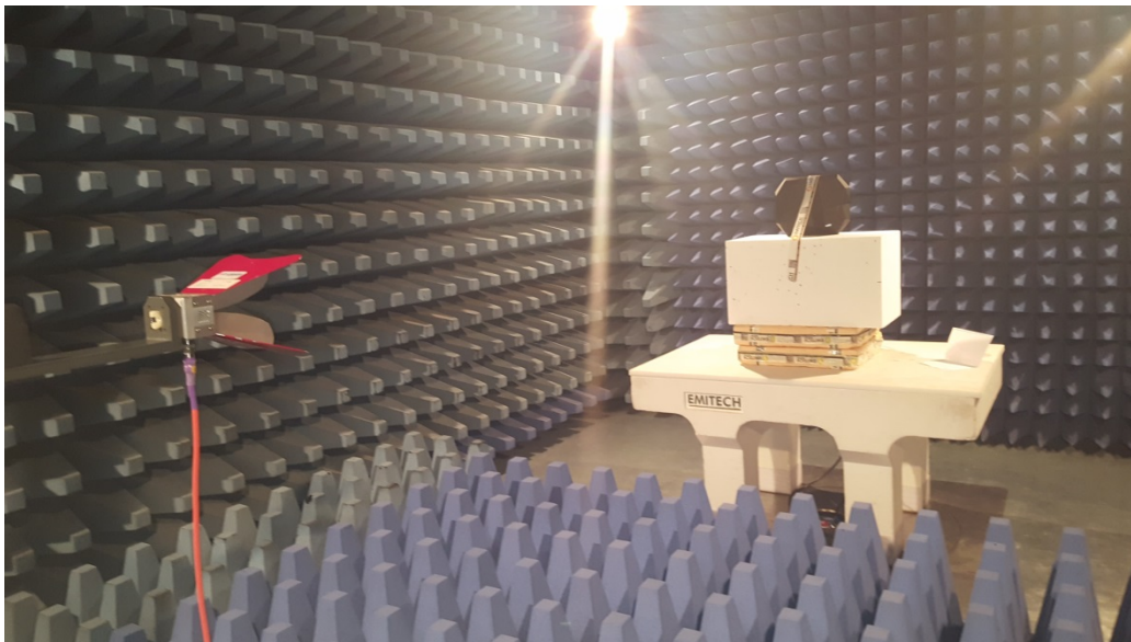
TEST SETUP PHOTO(S) - F > 1\text{GHz}
