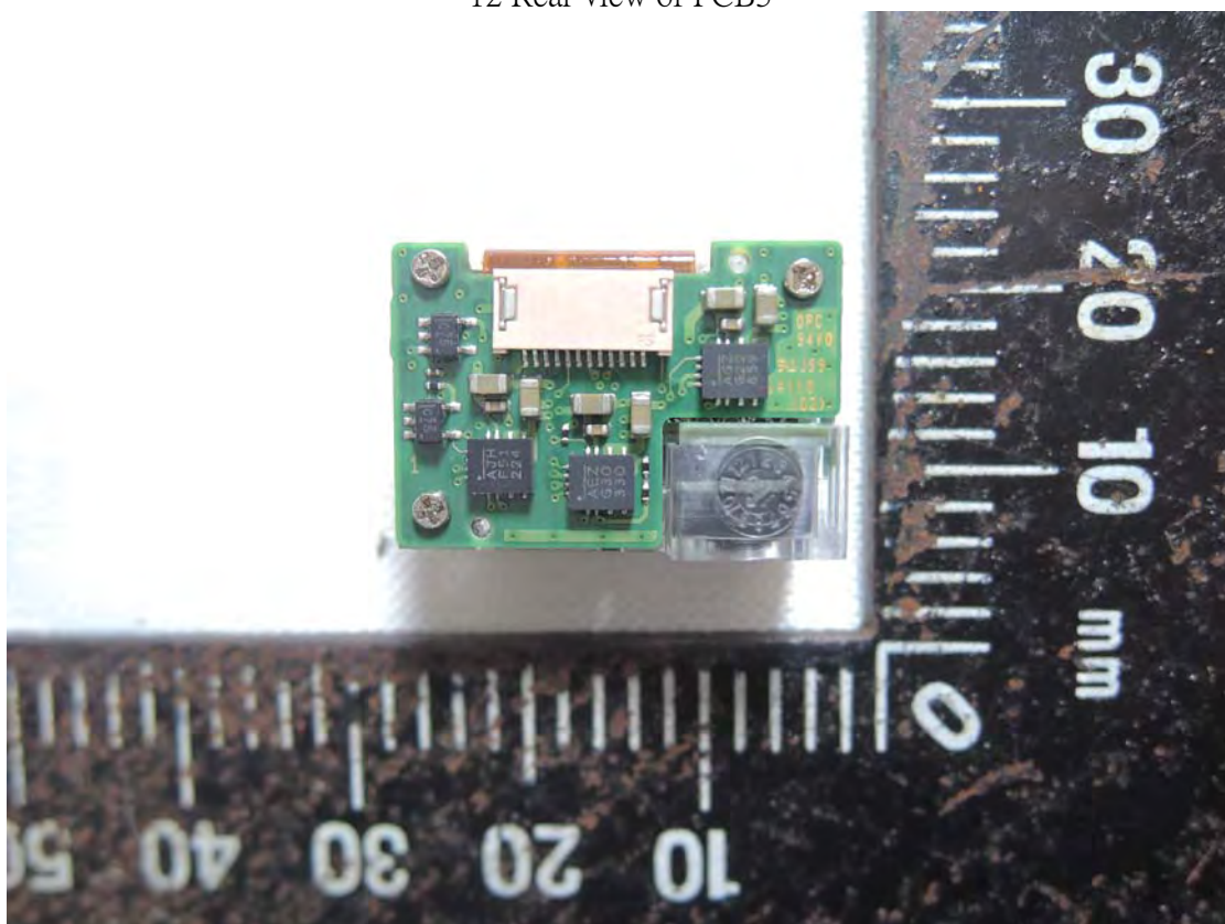
12 Rear view of PCB3
