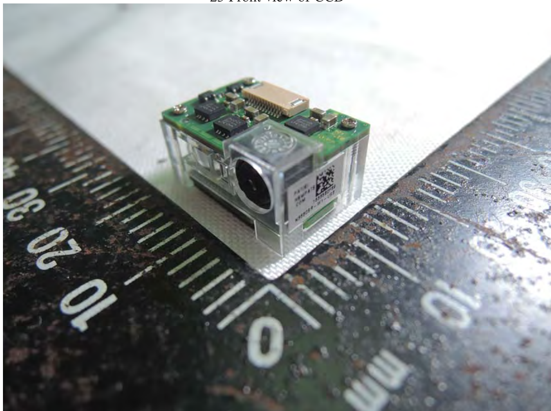
23 Front view of CCD
