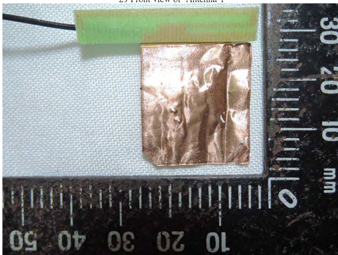
29 Front view of Antenna-1
