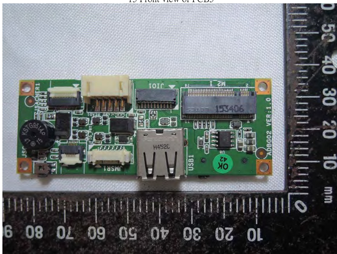
15 Front view of PCB5
