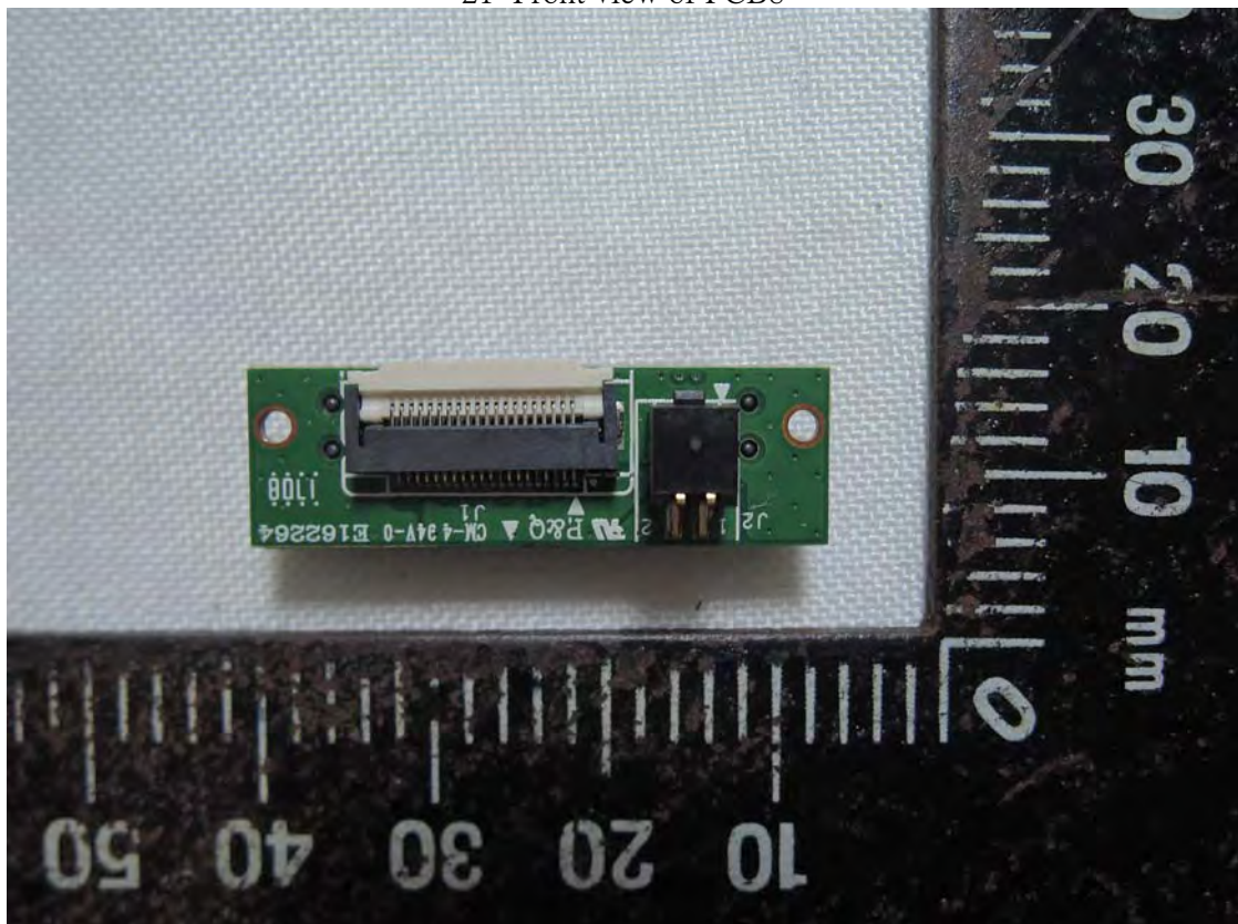
21 Front view of PCB8
