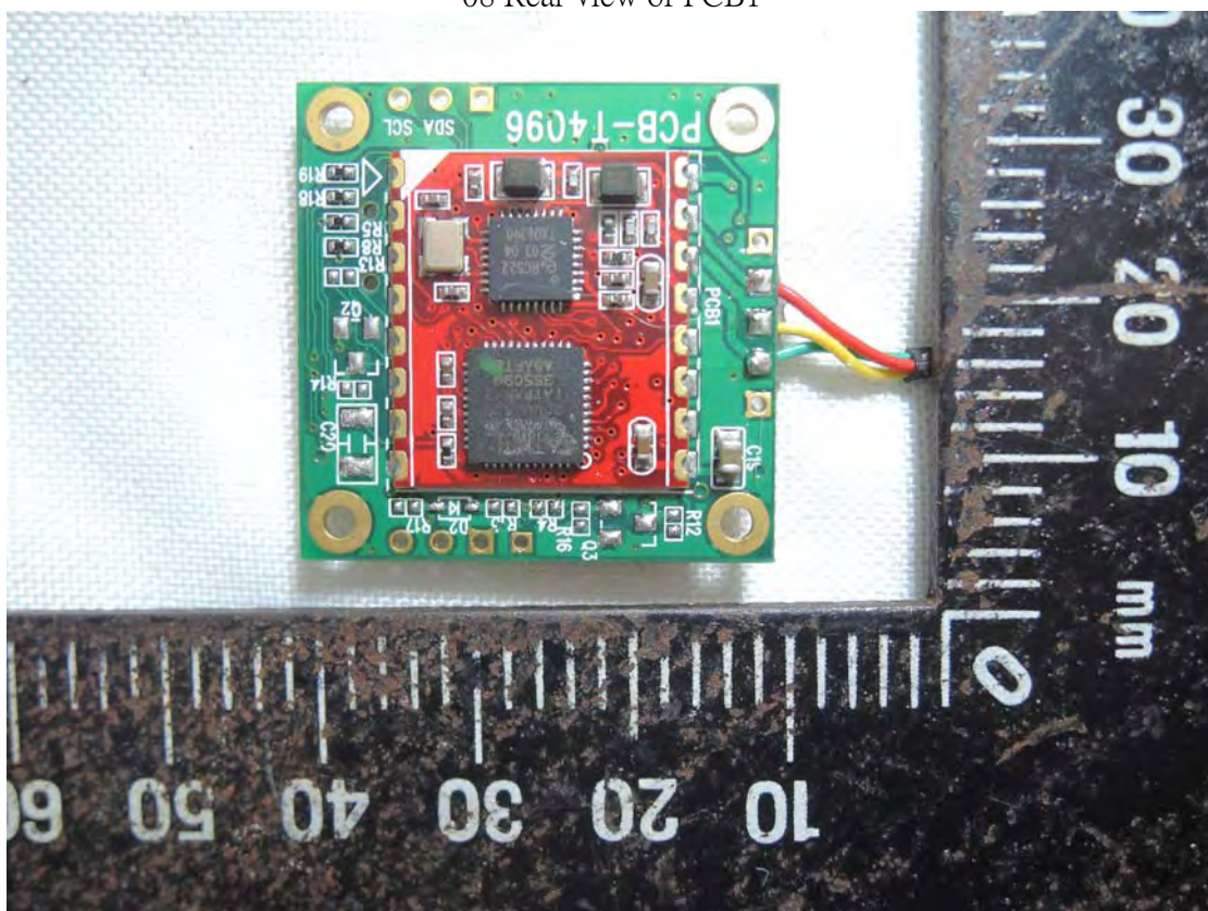
08 Rear view of PCB1
