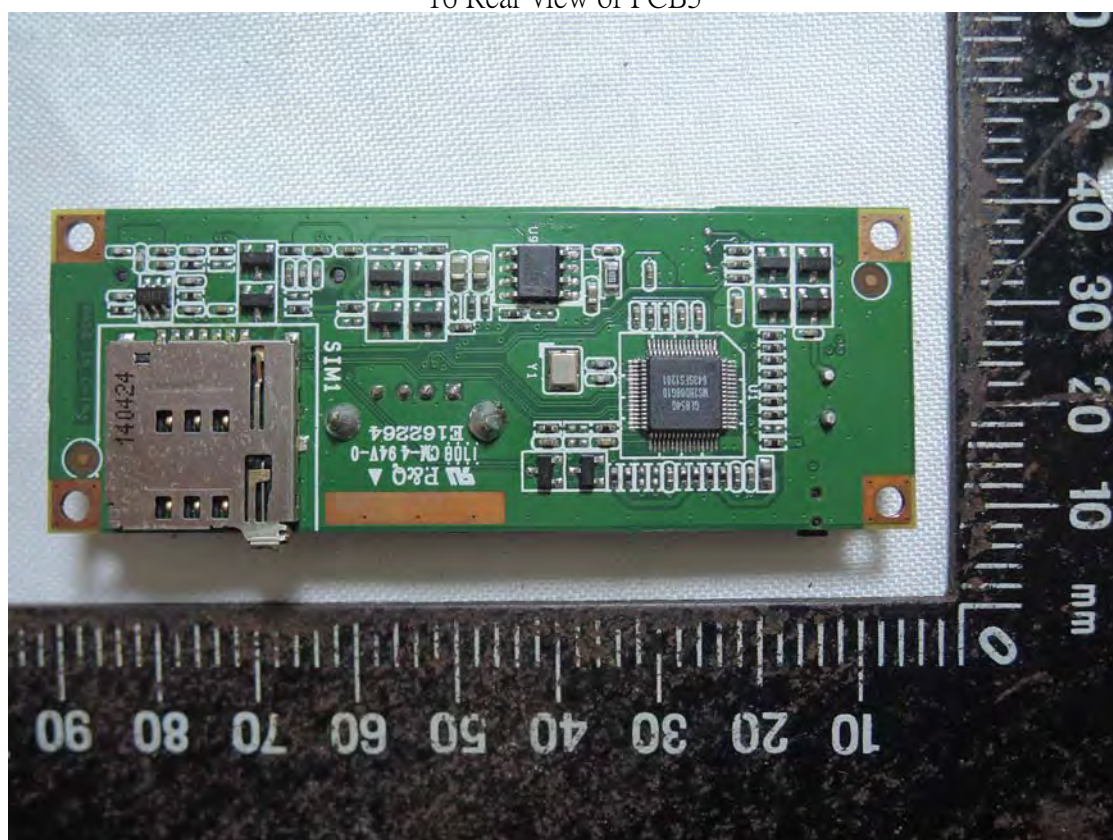
16 Rear view of PCB5
