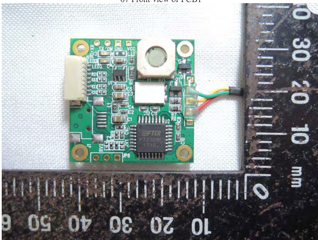
07 Front view of PCB1
