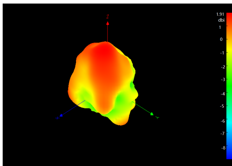
Antenna Radiation Pattern 3D (5750MHz)
