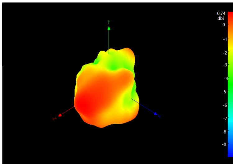
Antenna Radiation Pattern 3D (5750MHz)
