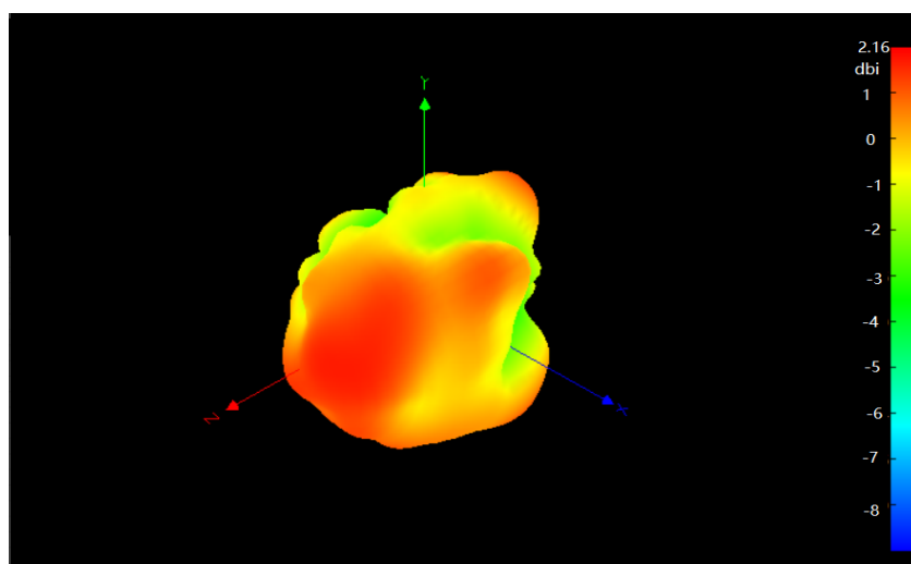
AntennaRadiationPattern3D (5750MHz)
