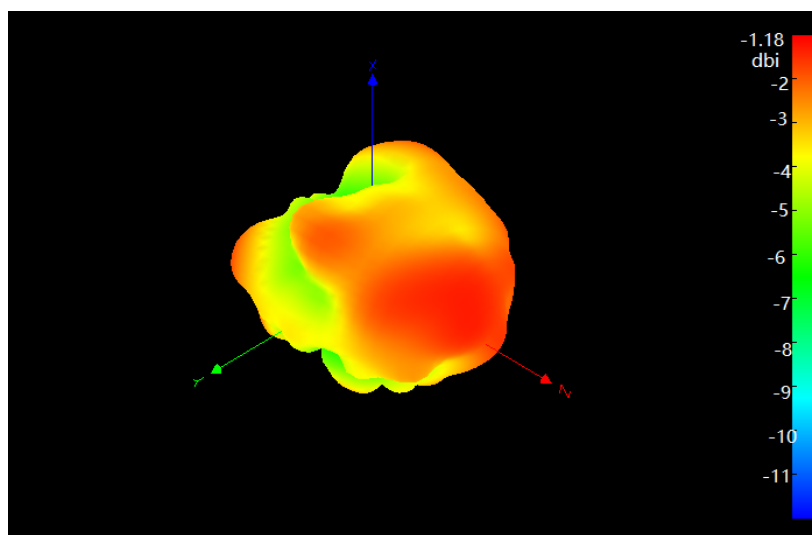
AntennaRadiationPattern3D (5750MHz)
