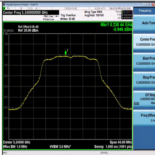
11AC20SISO-Ant2-5240-PASS
