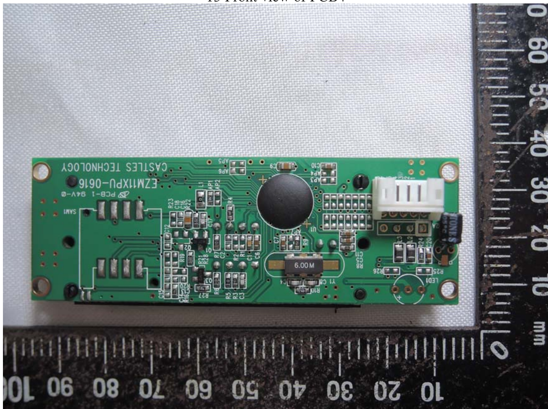
13 Front view of PCB4
