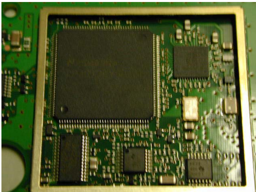
Figure 3: View of shielding area
