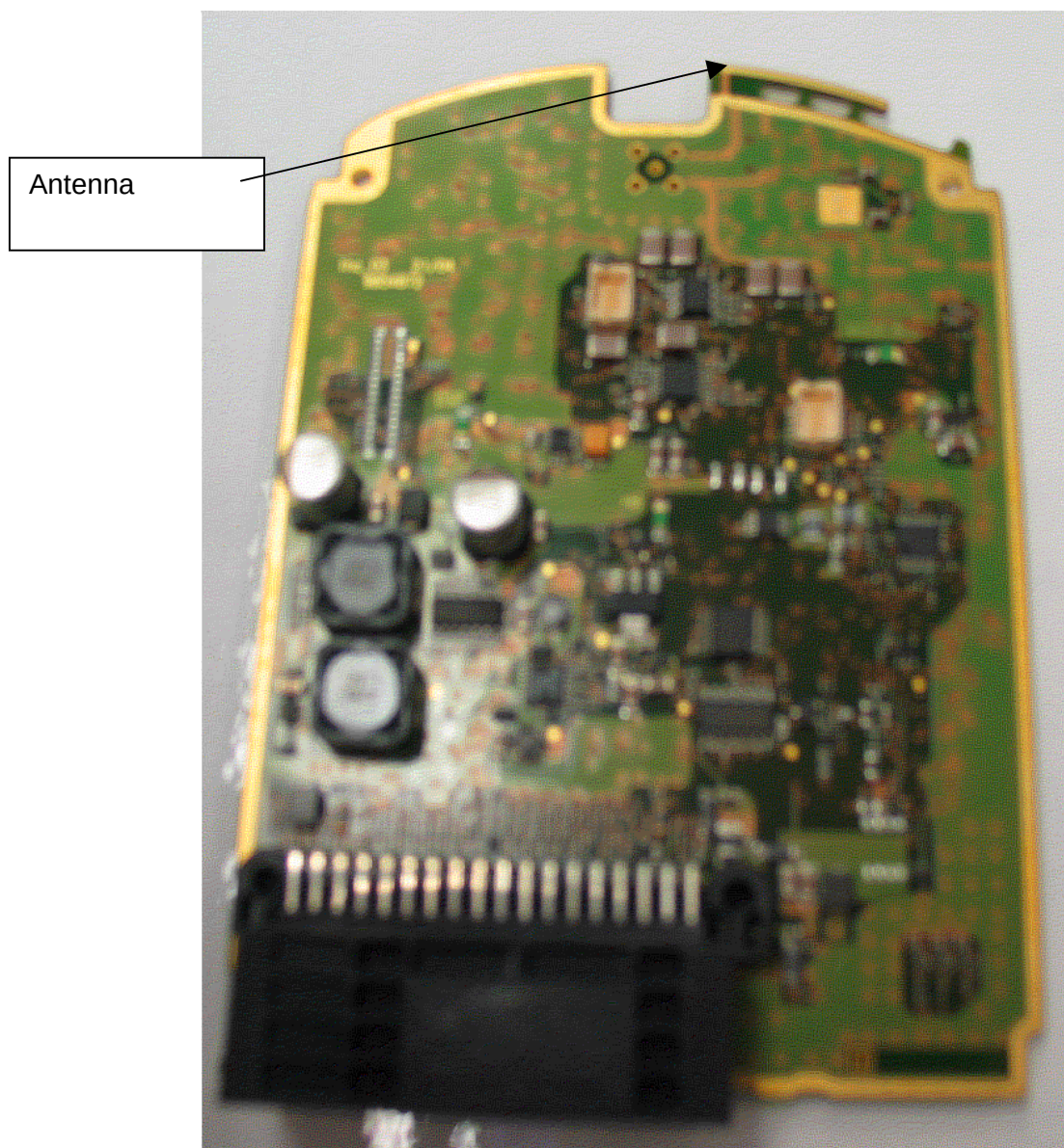
Figure 1: Top view of PWB
