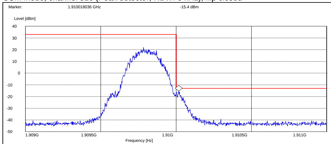
GSM mode, channel 810 (Peak detector, RBW: 3 kHz), flip closed
