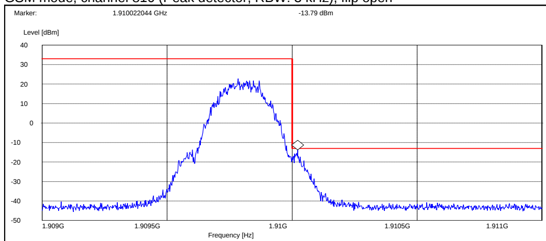
GSM mode, channel 810 (Peak detector, RBW: 3 kHz), flip open
