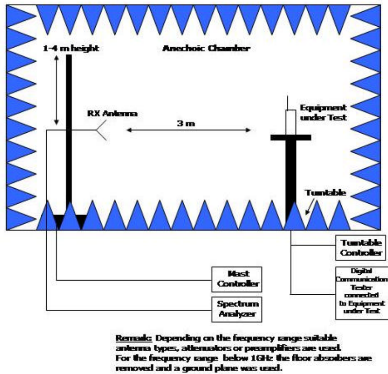
Drawing 2 : Setup for radiated emission measurement (anechoic chamber, in principle)
