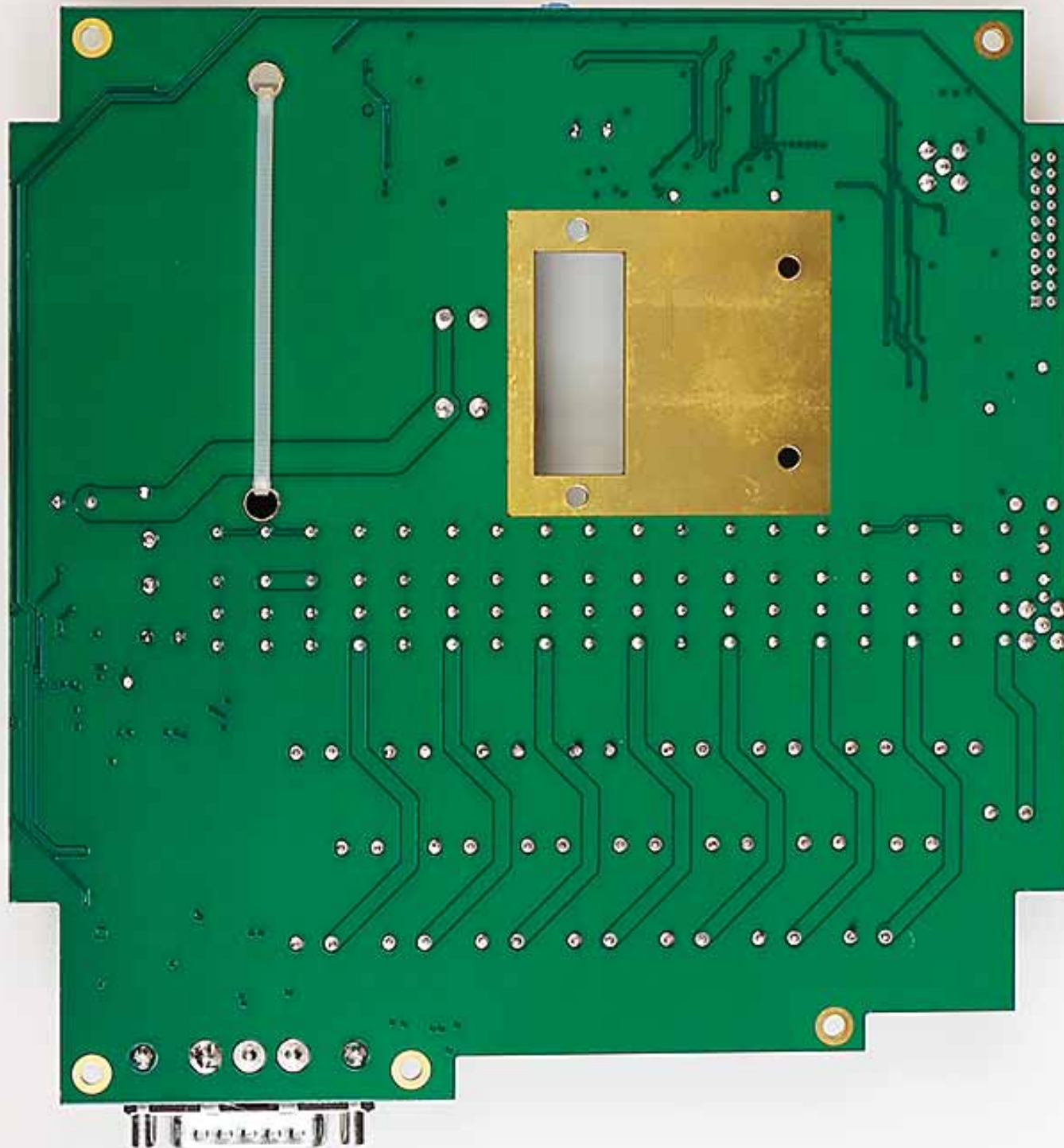
Power supply and PA board - Bottom
