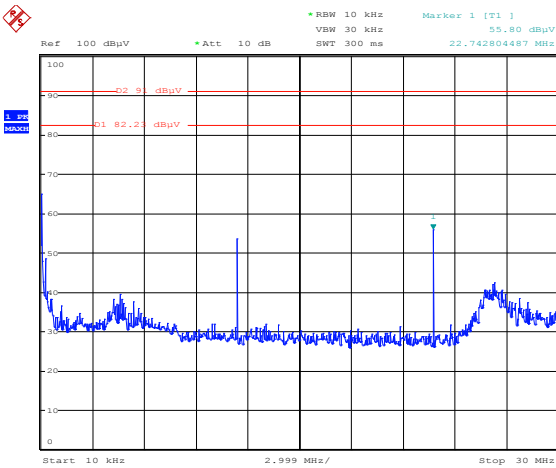
Figure 8.6-1: Low channel Radiated Spurious 125W
