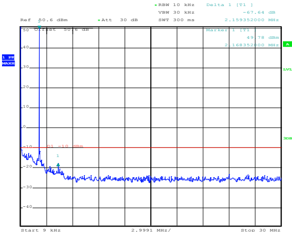
Figure 8.5-5: Mid channel Conducted Spurious 125W 1800 Hz and 400 Hz
