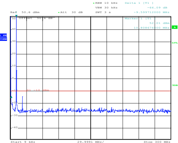
Figure 8.5-6: High channel Conducted Spurious 125W 1800 Hz and 400 Hz
