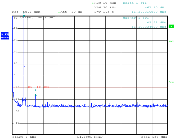
Figure 8.5-9: High channel Conducted Spurious 150W 1500 Hz
