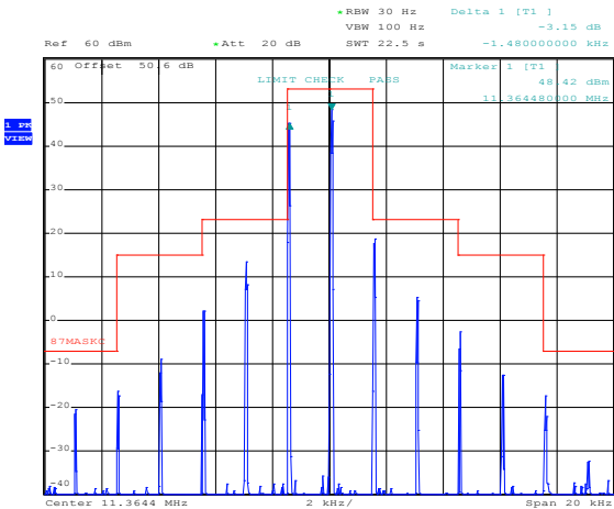
Figure 8.3-9: High channel Mask 150W 400 Hz and 1800 Hz
