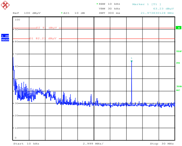
Figure 8.6-9: Mid channel Radiated Spurious 150W
