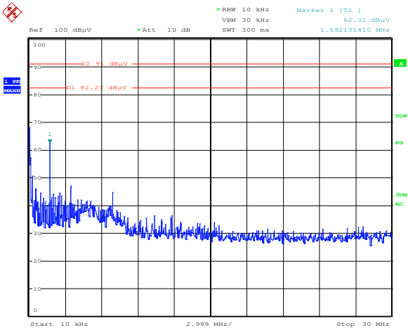
Figure 8.5-5: High channel Radiated Spurious 125W
