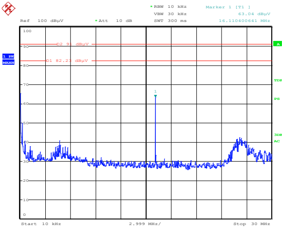
Figure 8.5-1: Low channel Radiated Spurious 125W
