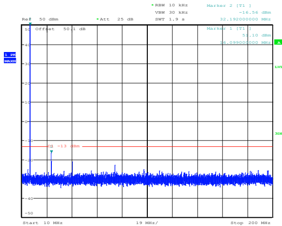
Figure 8.4-6: High channel Mask 125W 400 Hz and 1800 Hz Conducted Spurious
