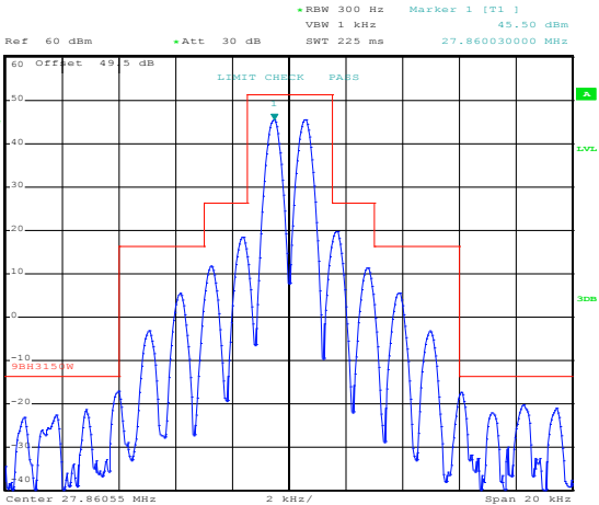
Figure 8.3-10: Low channel Mask 150W 1100 Hz
