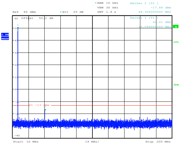
Figure 8.4-9: High channel Mask 150W 1500 Hz Conducted Spurious
