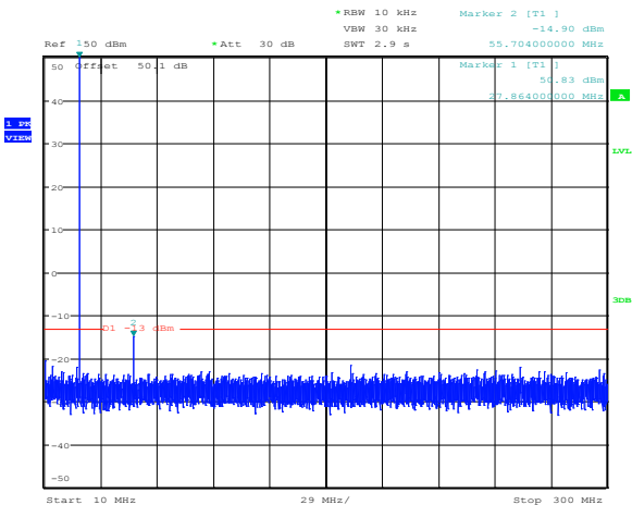
Figure 8.4-1: Low channel Mask 150W 400 Hz and 1800 Hz Conducted Spurious
