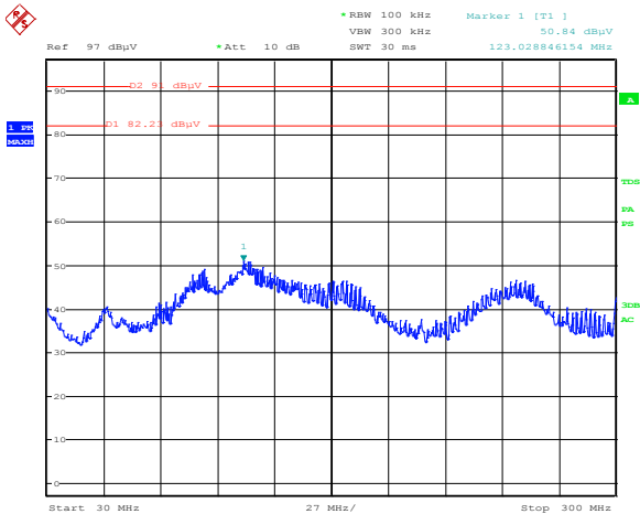
Figure 8.5-6: High channel Radiated Spurious 125W
