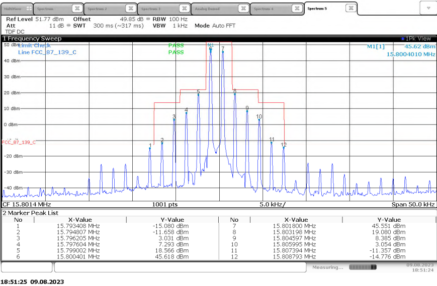
Figure 2.4.6-5 - Emissions Mask – 15.8 MHz – J3E
