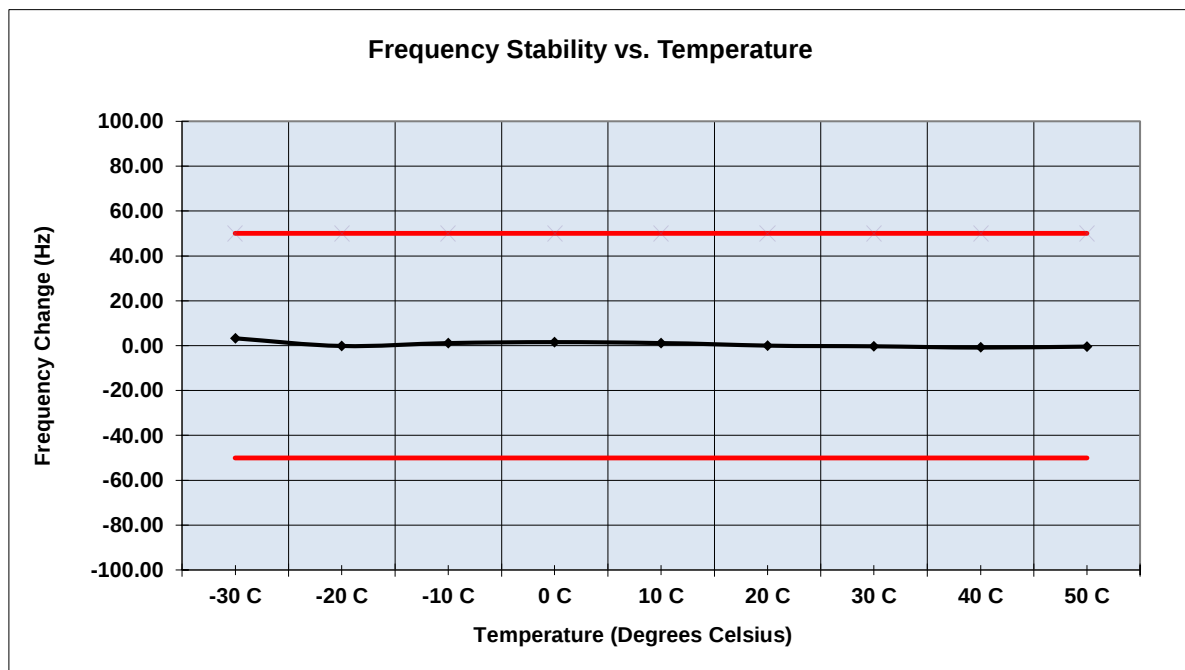
Figure 2.7.6-2 - Frequency Stability – 15.8 MHz – 13.8 VDC
