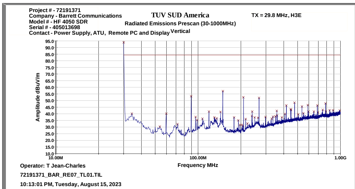
Figure 2.6.6-3 - Transmitter Radiated Spurious Emissions Representative Scan Plot – 29.8 MHz - H3E – 30 MHz – 1 GHz – Vertical Polarization
