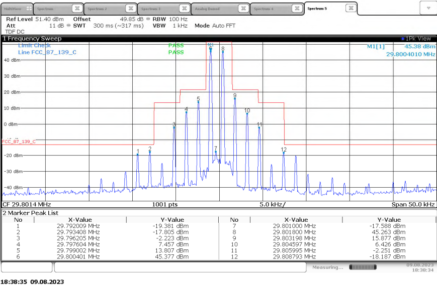
Figure 2.4.6-6 - Emissions Mask – 29.8 MHz – J3E
