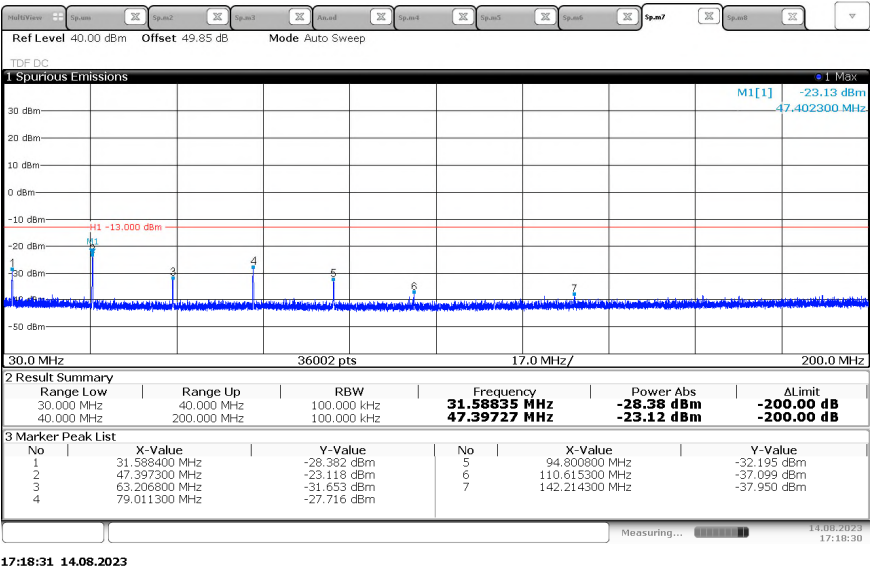
Figure 2.5.6-13 - Transmitter Conducted Spurious Emissions – 15.8 MHz – J3E
