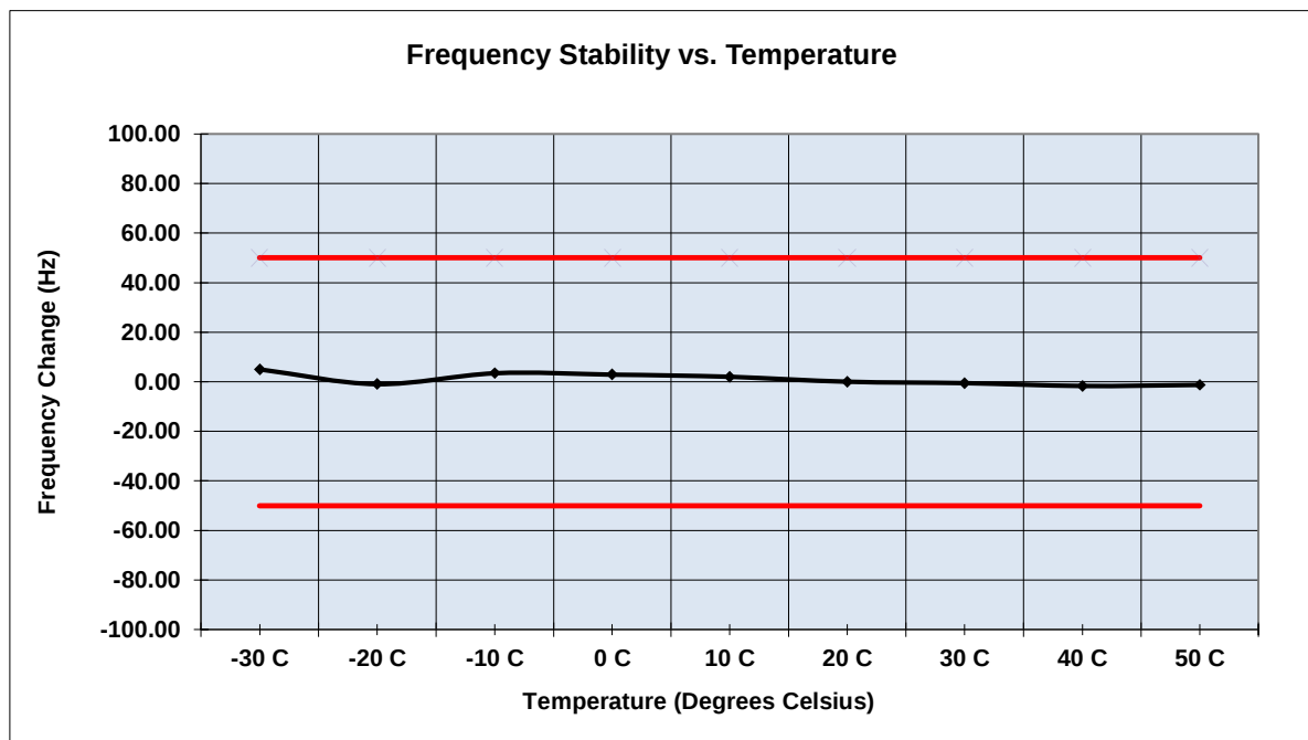
Figure 2.7.6-3 - Frequency Stability – 29.8 MHz – 13.8 VDC
