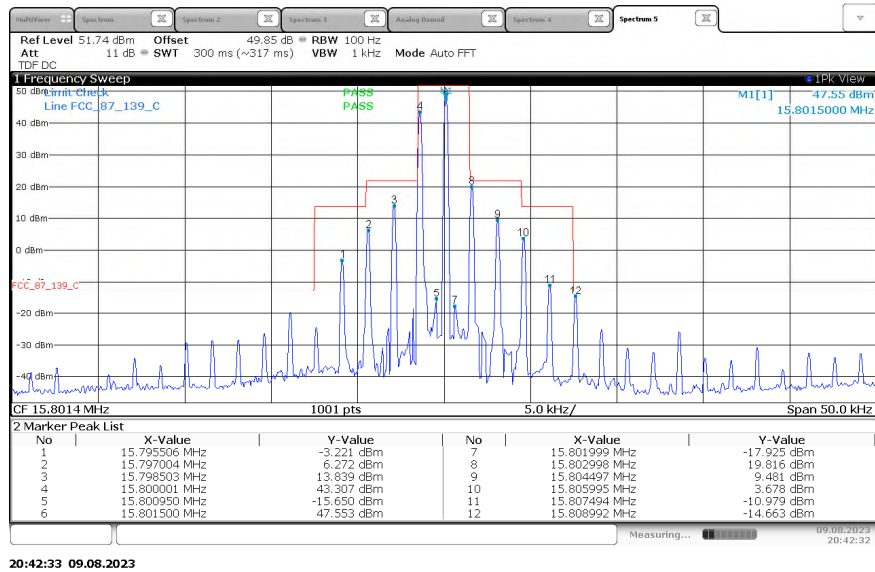
Figure 2.4.6-2 - Emissions Mask – 15.8 MHz – H3E
