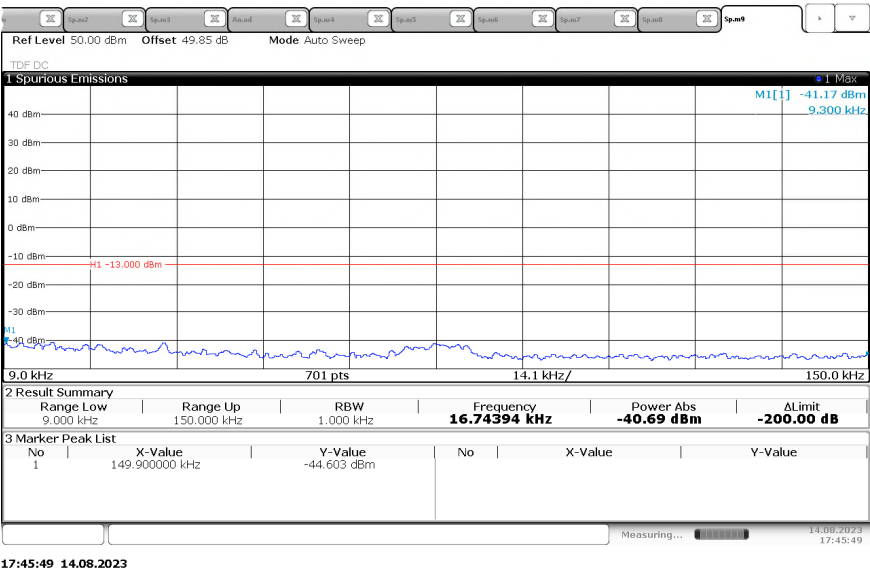
Figure 2.5.6-14 - Transmitter Conducted Spurious Emissions – 29.8 MHz – J3E
