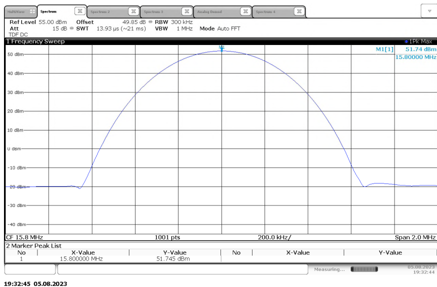
Figure 2.1.6-2 - RF Output Power – 15.8 MHz – H3E
