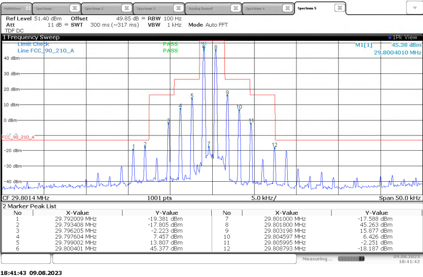
Figure 2.4.6-12 - Emissions Mask – 29.8 MHz – J3E
