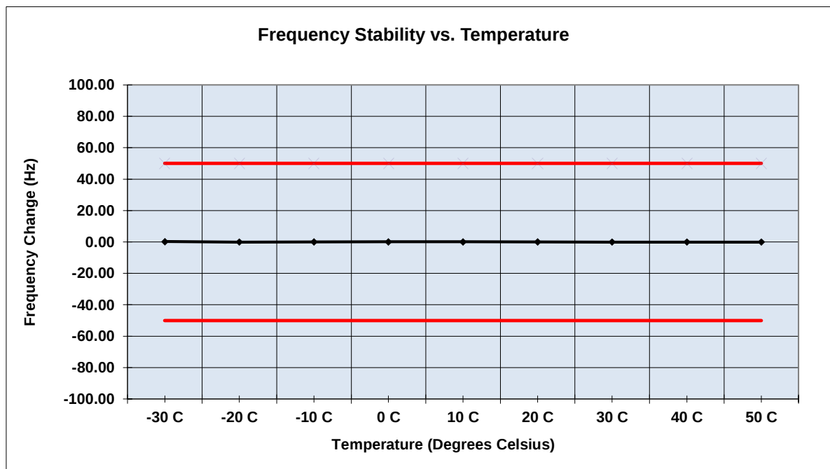
Figure 2.7.6-4 - Frequency Stability – 1.6 MHz – 24 VDC
