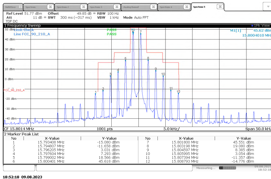
Figure 2.4.6-11 - Emissions Mask – 15.8 MHz – J3E
