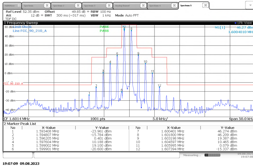
Figure 2.4.6-10 - Emissions Mask – 1.6 MHz – J3E
