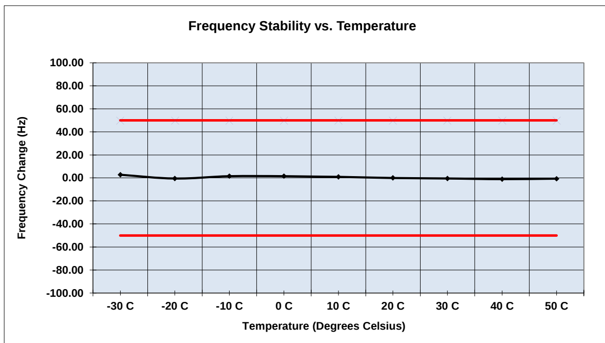
Figure 2.7.6-5 - Frequency Stability – 15.8 MHz – 24 VDC
