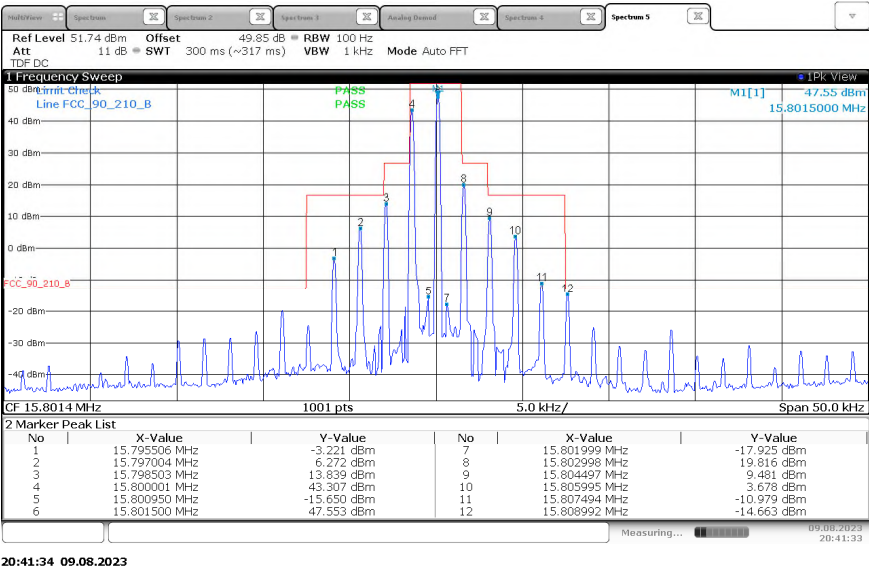
Figure 2.4.6-8 - Emissions Mask – 15.8 MHz – H3E
