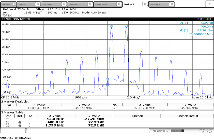
Figure 2.3.6-13 – Modulation Characteristics – Carrier Attenuation – J3E – 15.8 MHz
