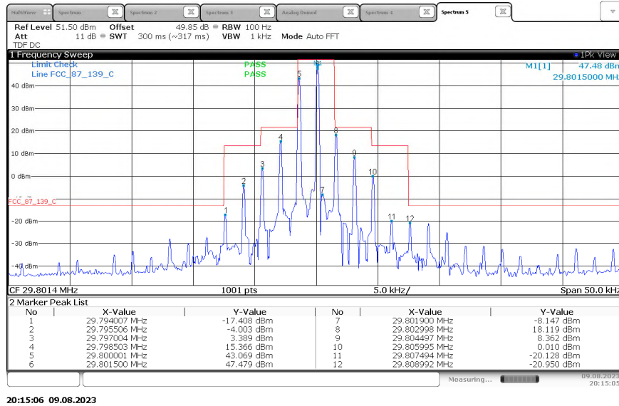
Figure 2.4.6-3 - Emissions Mask – 29.8 MHz – H3E
