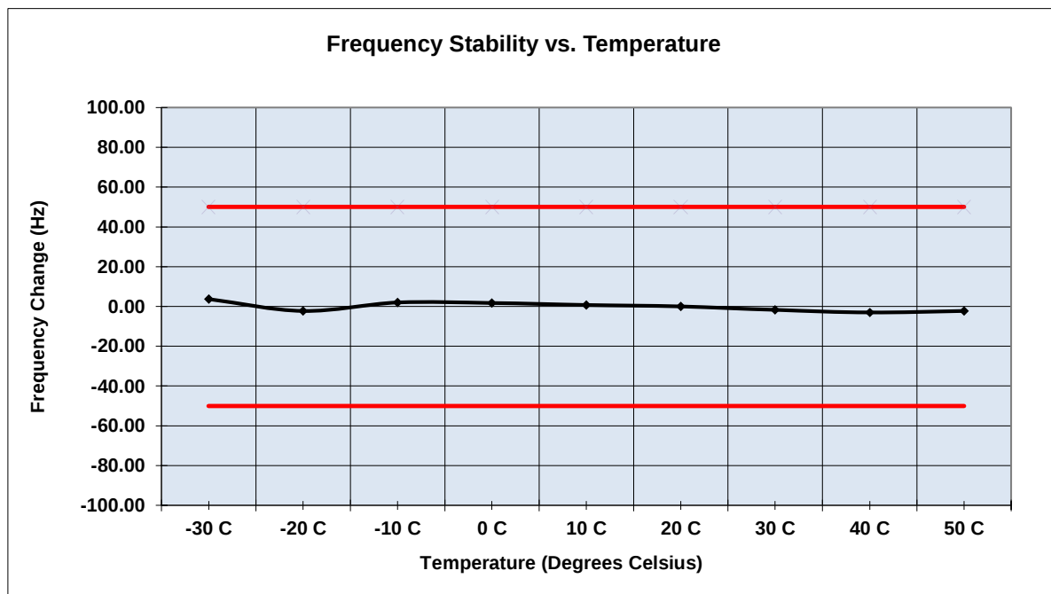
Figure 2.7.6-6 - Frequency Stability – 29.8 MHz – 24 VDC
