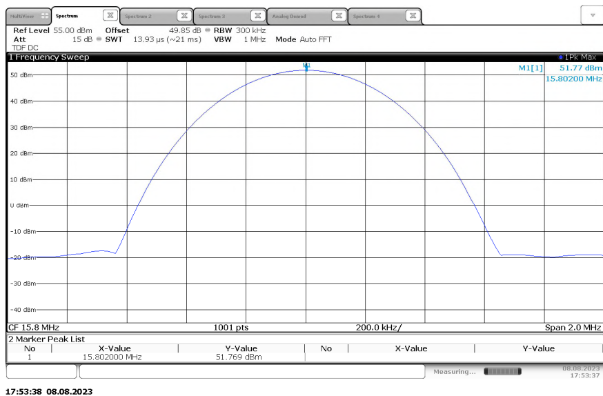
Figure 2.1.6-5 - RF Output Power – 15.8 MHz – J3E
