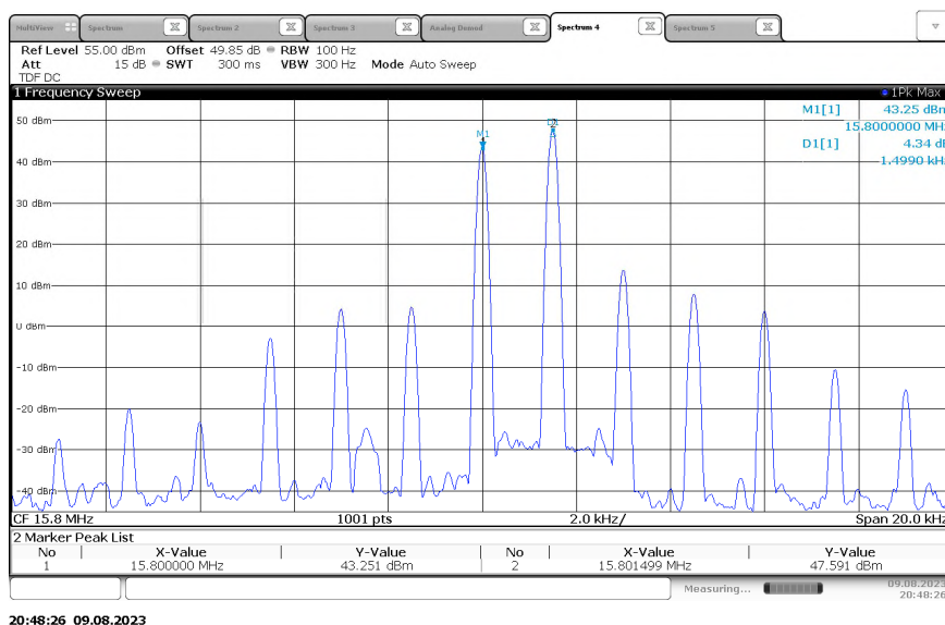
Figure 2.3.6-10 – Modulation Characteristics – Carrier Attenuation – H3E – 15.8 MHz
