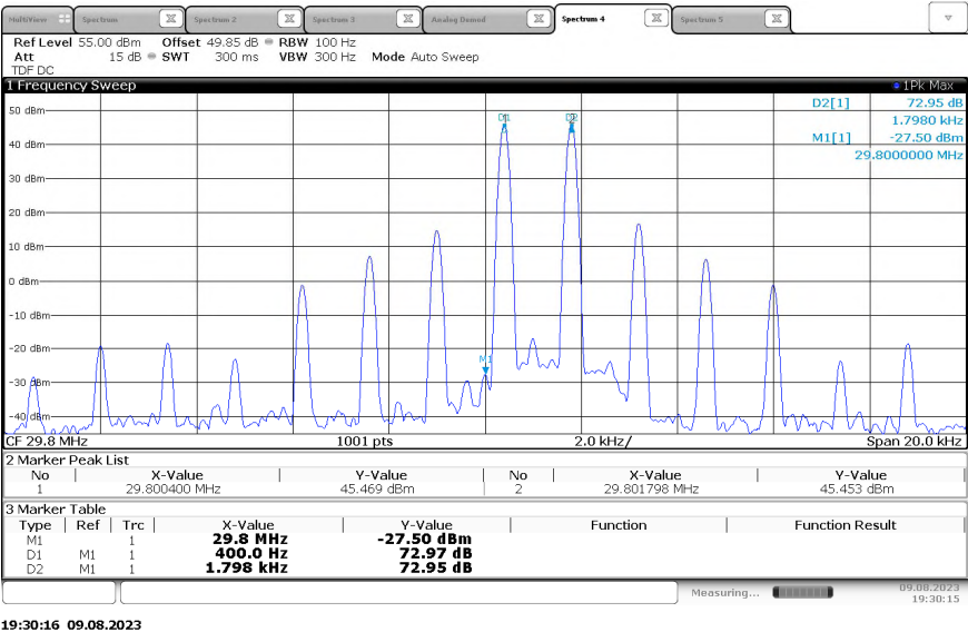
Figure 2.3.6-14 – Modulation Characteristics – Carrier Attenuation – J3E – 29.8 MHz
