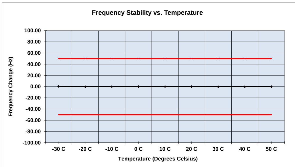
Figure 2.7.6-1 - Frequency Stability – 1.6 MHz – 13.8 VDC
