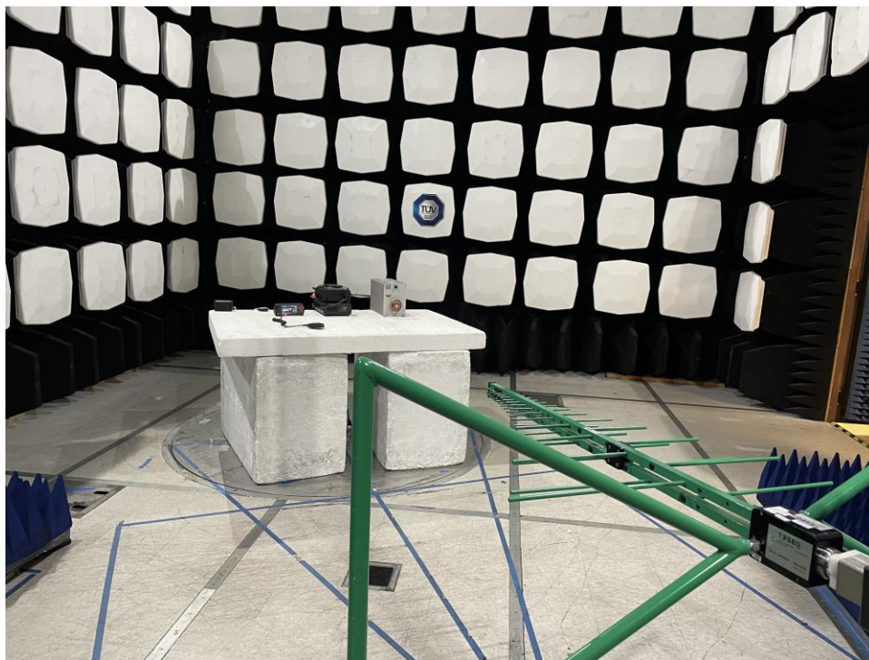
Figure A-3: Test Setup – Front View of the Radiated Emissions 30 – 500 MHz
