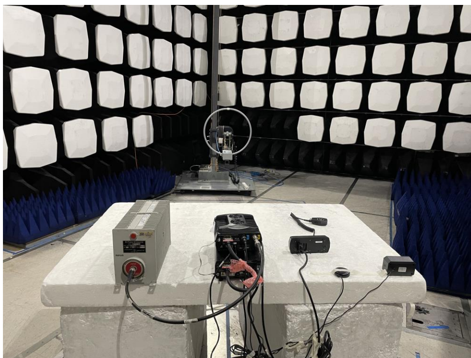
Figure A-2: Test Setup – Rear view of the Radiated Emissions 9kHz - 30 MHz
