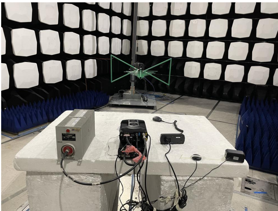
Figure A-4: Test Setup – Rear View of the Radiated Emissions 30 – 500 MHz
