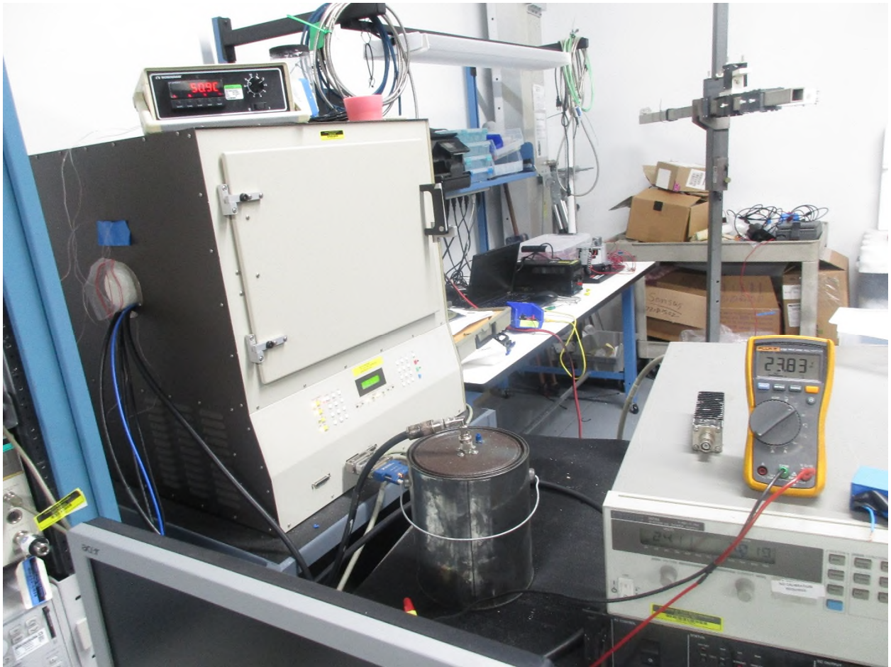
Figure 8: Frequency Stability
