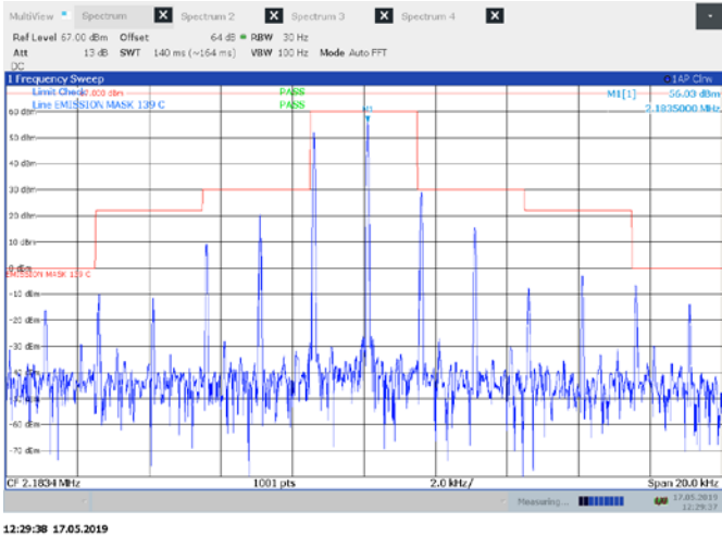
Figure 8.3-4: Low channel Mask 1000W H3E
