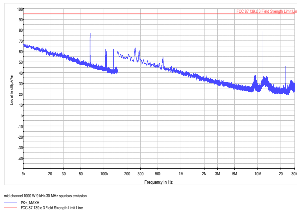
Figure 8.6-3: Mid channel Radiated Spurious 1000W 9 kHz-30 MHz
