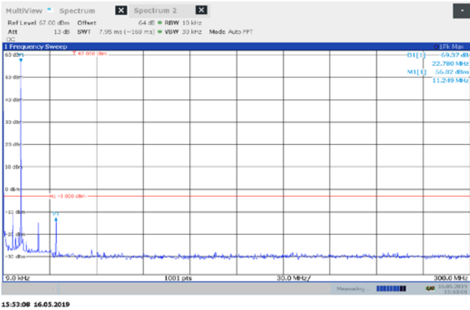
Figure 8.5-5: Mid channel Conducted Spurious 1000W J3E
