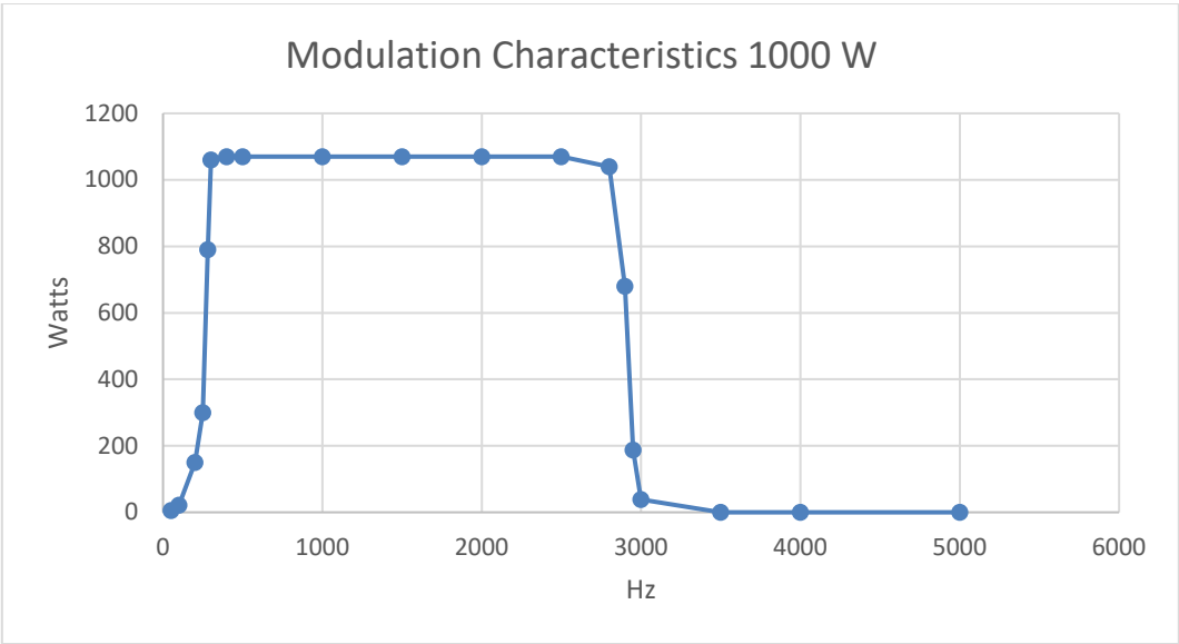
Figure 8.2-1: Modulation Characteristic 1000 Watts
