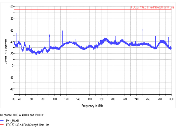
Figure 8.6-4: Mid channel Radiated Spurious 1000W 30-300 MHz
