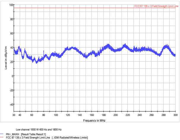
Figure 8.6-2: Low channel Radiated Spurious 1000W 30-300 MHz
