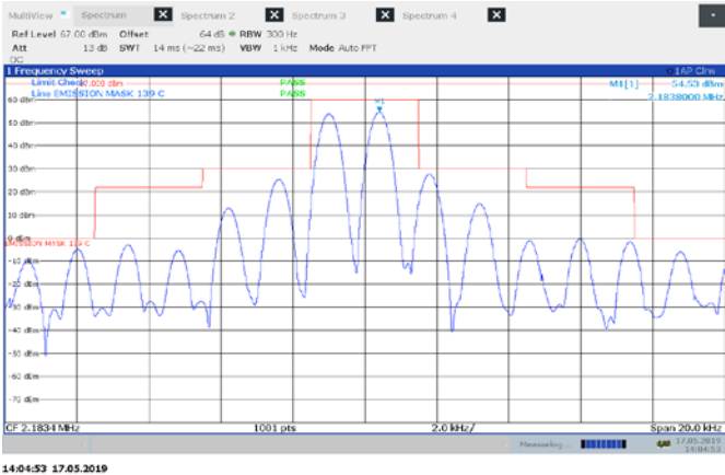
Figure 8.3-1: Low channel Mask 1000W J3E
