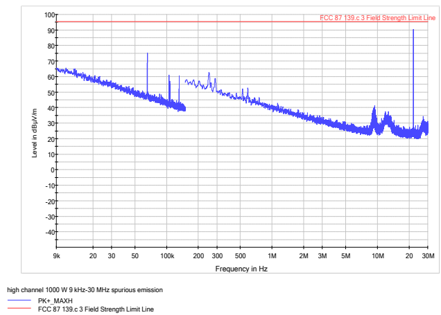
Figure 8.6-5: High channel Radiated Spurious 1000W 9 kHz-30 MHz
