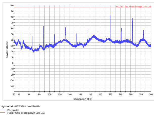
Figure 8.6-6: High channel Radiated Spurious 1000W 30-300 MHz
