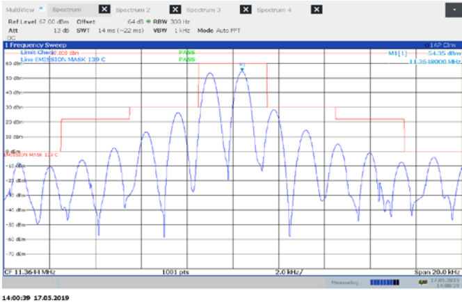
Figure 8.3-2: Mid channel Mask 1000W J3E
