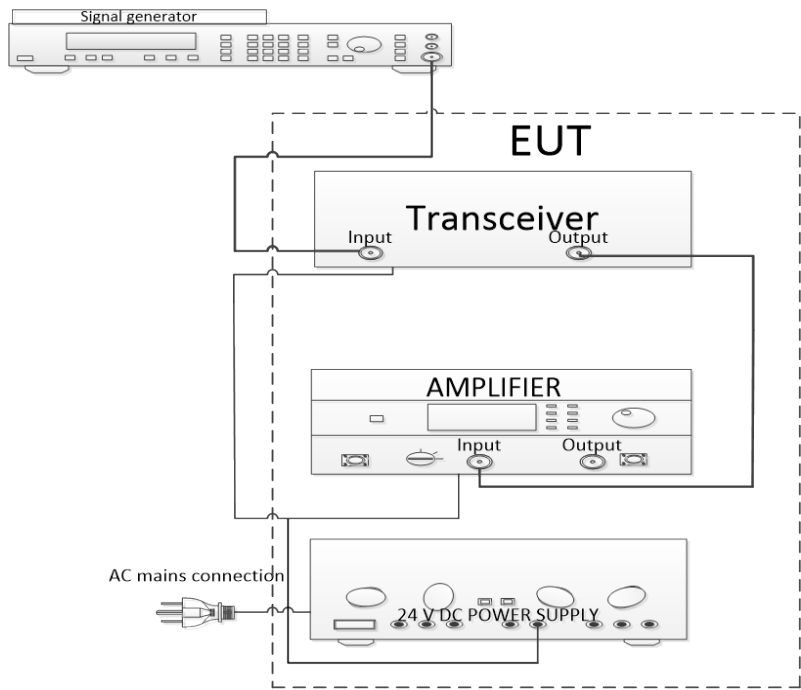
Figure 3.6-1: Setup diagram
