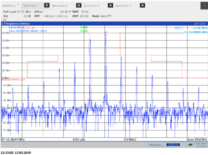
Figure 8.3-5: : Mid channel Mask 1000W H3E
