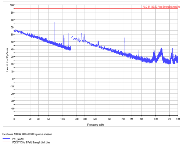
Figure 8.6-1: Low channel Radiated Spurious 1000W 9 kHz-30 MHz
