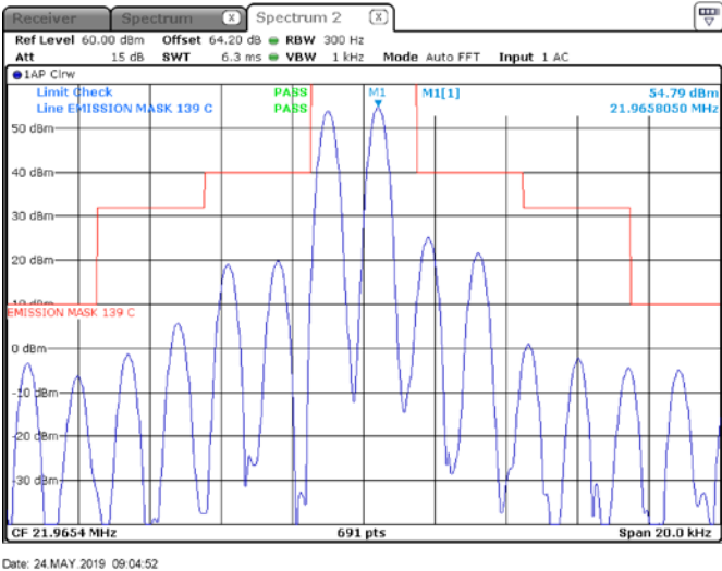
Figure 8.3-3: High channel Mask 1000W J3E
