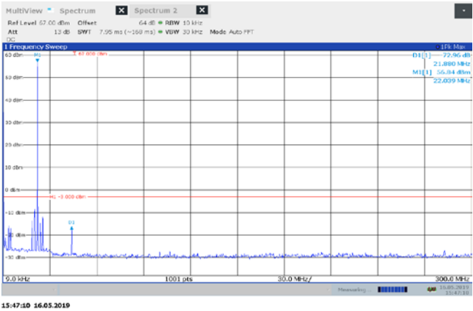
Figure 8.5-6: High channel Conducted Spurious 1000W J3E
