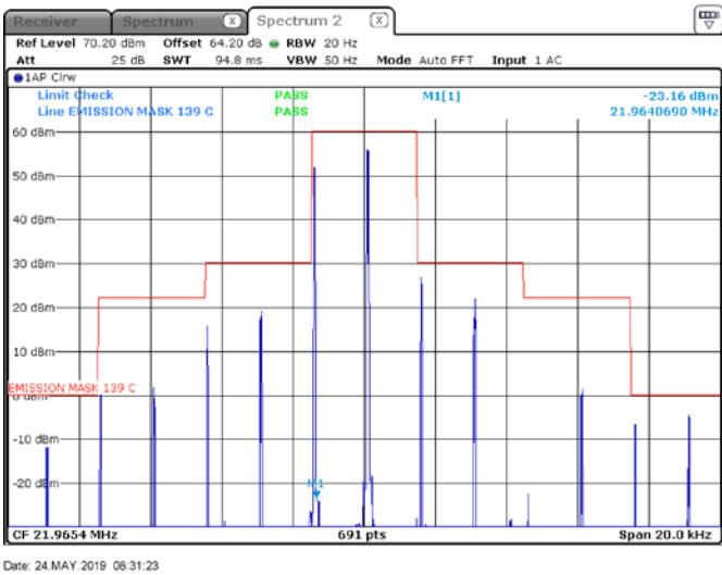
Figure 8.3-6: High channel Mask 1000W H3E
