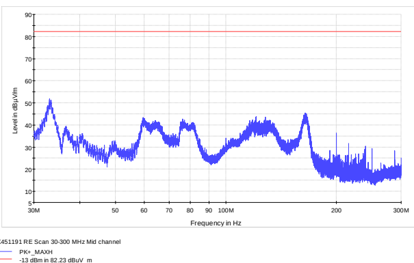
Figure 8.6-4: Mid channel Radiated Spurious
