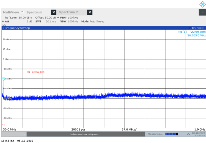
Figure 8.5-5: High channel 27.86 MHz, H3E modulation, Conducted Spurious
