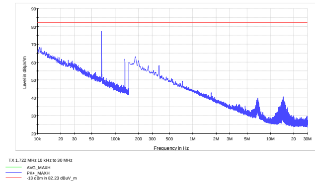
Figure 8.6-1: Low channel Radiated Spurious
