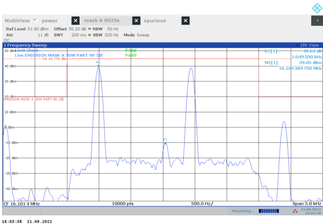
Figure 8.4-2: Mid channel 30W 400 Hz and 1800 Hz 40 dB Carrier suppression
