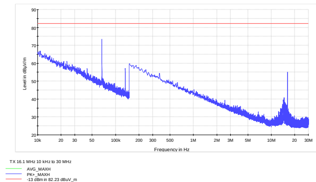
Figure 8.6-3: Mid channel Radiated Spurious
