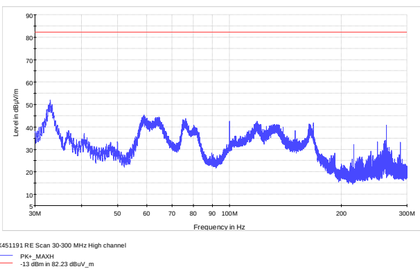
Figure 8.6-6: High channel Radiated Spurious
