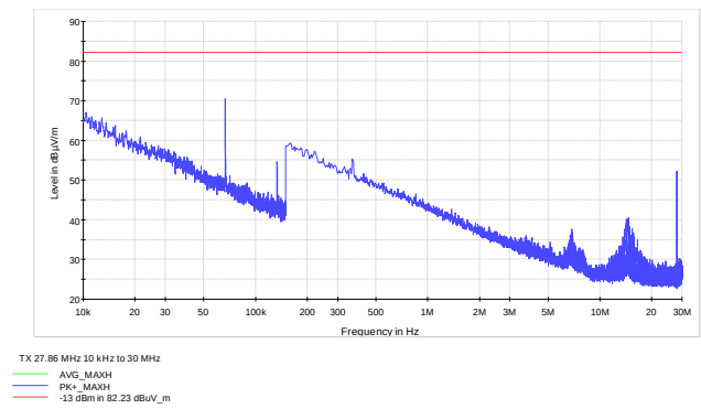
Figure 8.6-5: High channel Radiated Spurious
