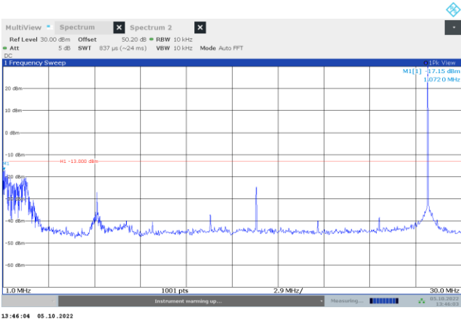
Figure 8.5-4: High channel 27.86 MHz, H3E modulation, Conducted Spurious
