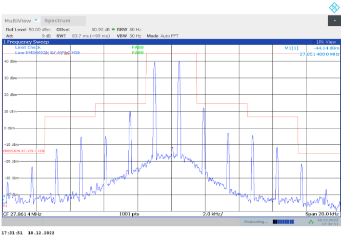
Figure 8.3-9: High channel 30W 400 Hz and 1800 Hz 40 dB Carrier suppression
