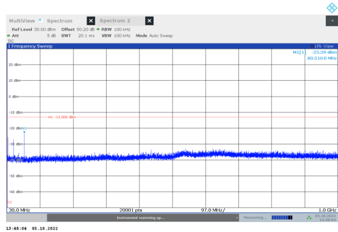
Figure 8.4-3: Mid channel 16.1 MHz, H3E modulation, Conducted Spurious
