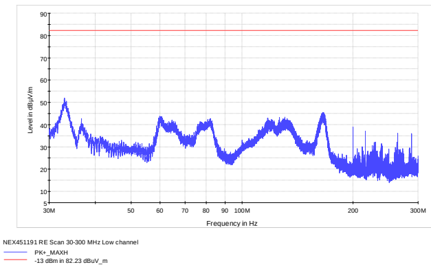
Figure 8.5-2: Low channel Radiated Spurious
