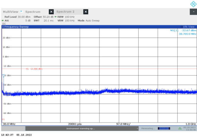
Figure 8.4-10: High channel 27.86 MHz, J3E modulation, Conducted Spurious
