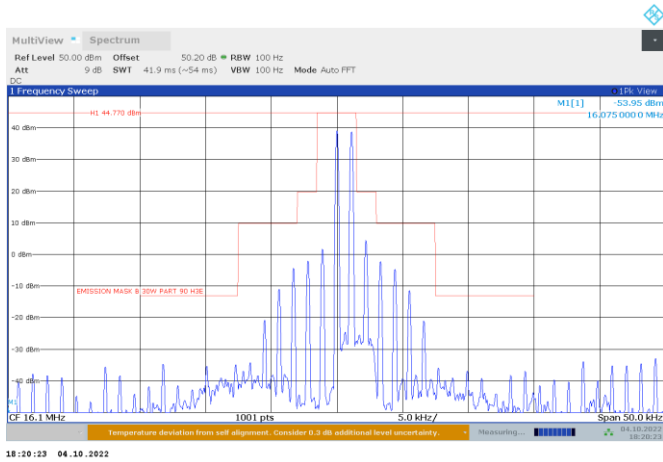
Figure 8.3-5: Mid channel Mask 30W 1500 Hz
