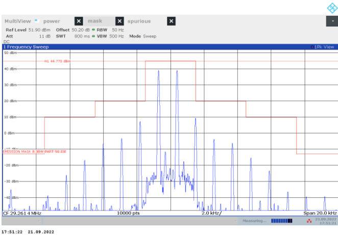
Figure 8.3-3: High channel Mask 30W 400 Hz and 1800 Hz
