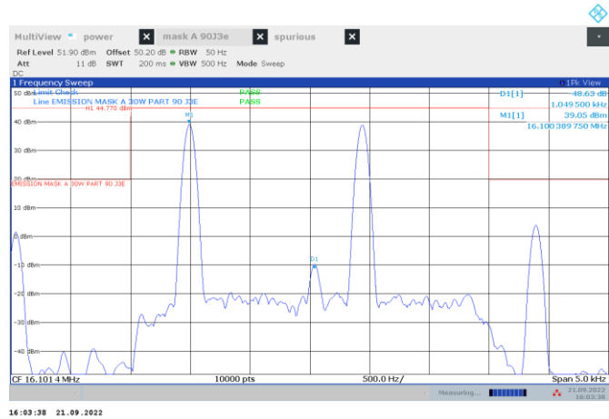
Figure 8.3-8: Mid channel 30W 400 Hz and 1800 Hz 40 dB Carrier suppression
