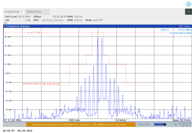
Figure 8.3-6: High channel Mask 30W 1500 Hz
