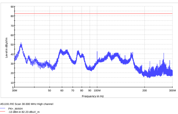
Figure 8.5-6: High channel Radiated Spurious
