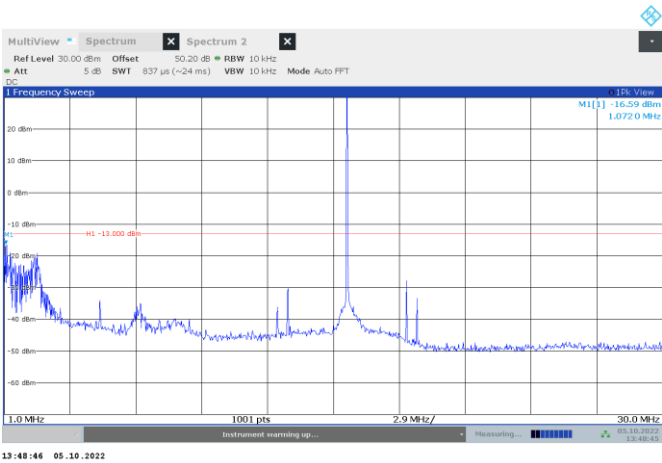
Figure 8.4-2: Mid channel 16.1 MHz, H3E modulation, Conducted Spurious
