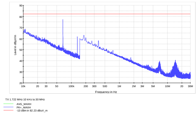
Figure 8.5-1: Low channel Radiated Spurious
