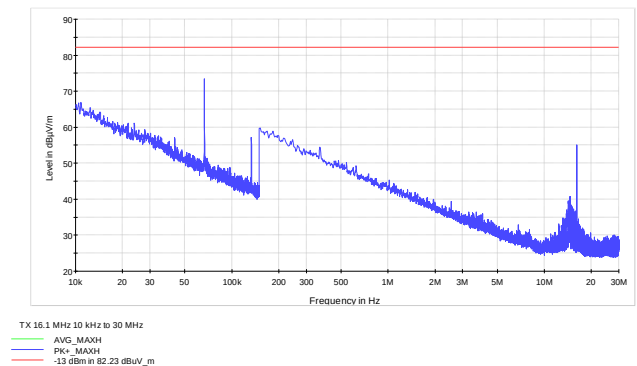
Figure 8.5-3: Mid channel Radiated Spurious
