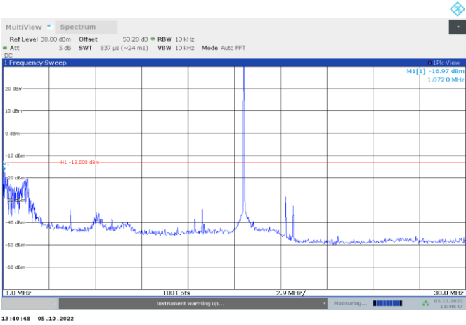
Figure 8.4-7: Mid channel 16.1 MHz, J3E modulation, Conducted Spurious
