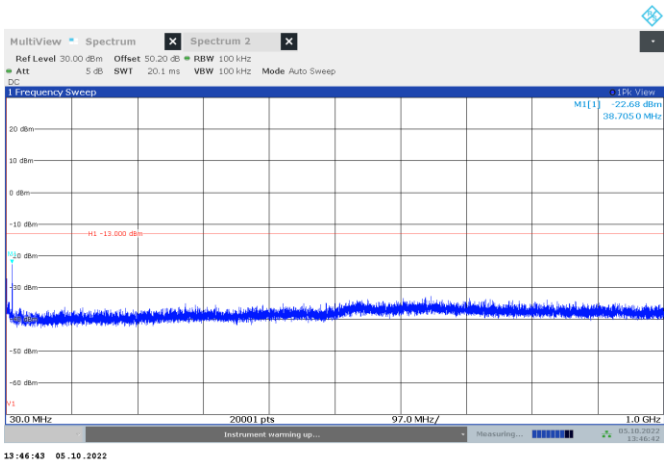
Figure 8.4-5: High channel 27.86 MHz, H3E modulation, Conducted Spurious
