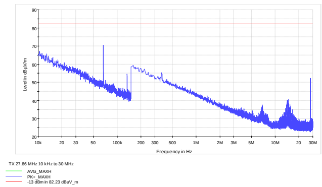
Figure 8.5-5: High channel Radiated Spurious
