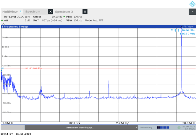
Figure 8.4-9: High channel 27.86 MHz, J3E modulation, Conducted Spurious
