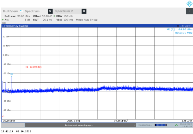
Figure 8.4-8: Mid channel 16.1 MHz, J3E modulation, Conducted Spurious
