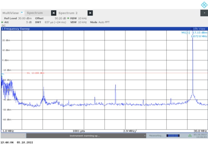
Figure 8.4-4: High channel 27.86 MHz, H3E modulation, Conducted Spurious
