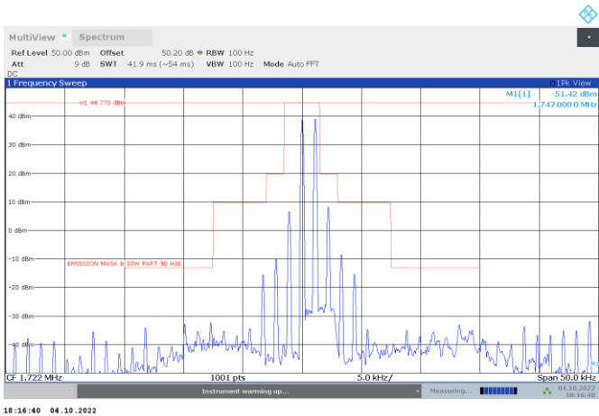
Figure 8.3-4: Low channel Mask 30W 1500 Hz
