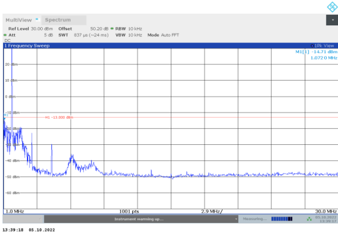
Figure 8.4-6: Low channel 1.722 MHz, J3E modulation, Conducted Spurious
