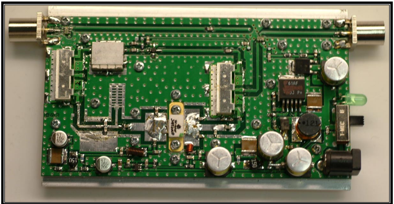
PHOTOGRAPH 13: PCB TOP VIEW
