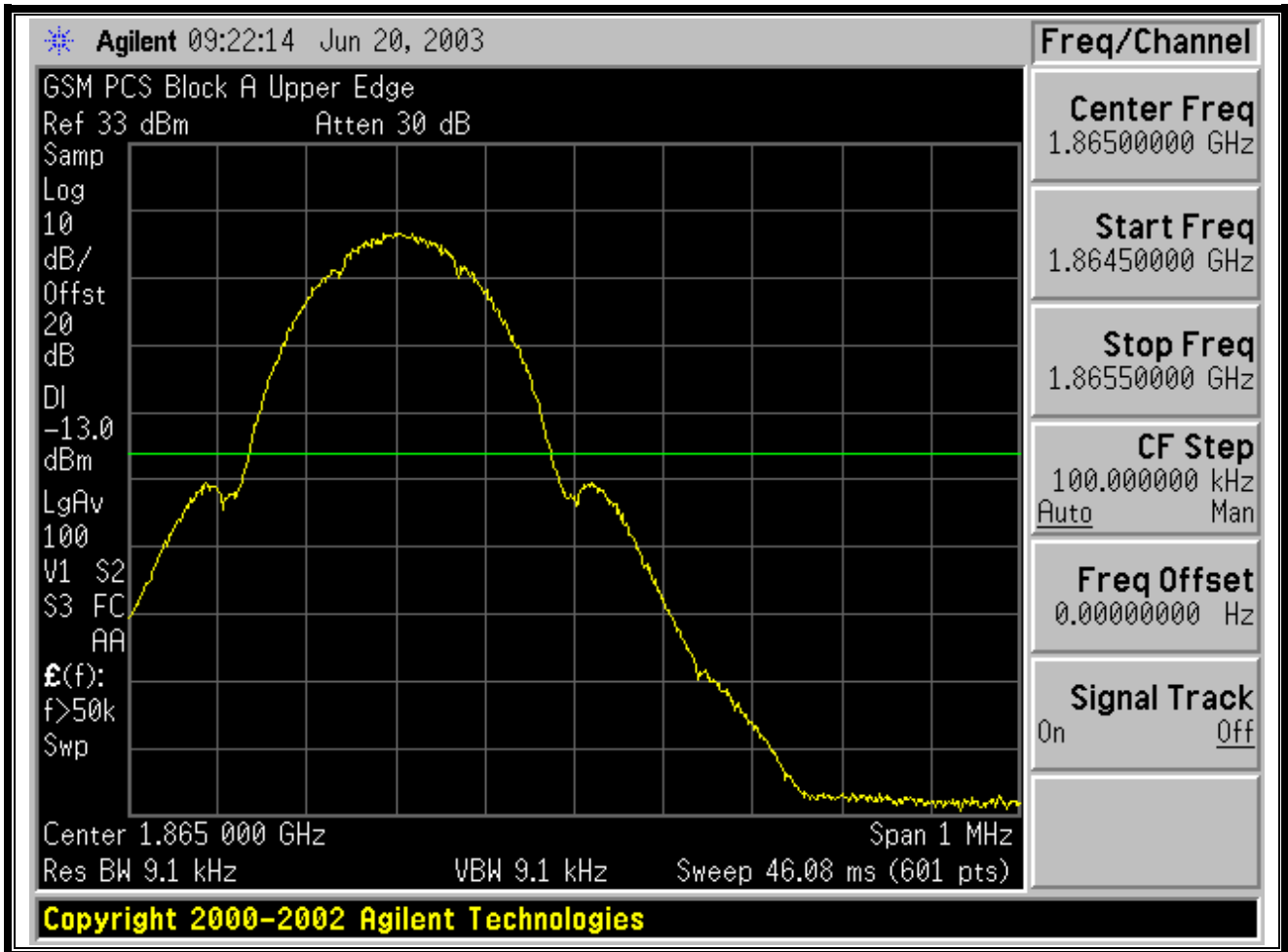
PLOT 11-2: GSM UPPER BAND EDGE A
