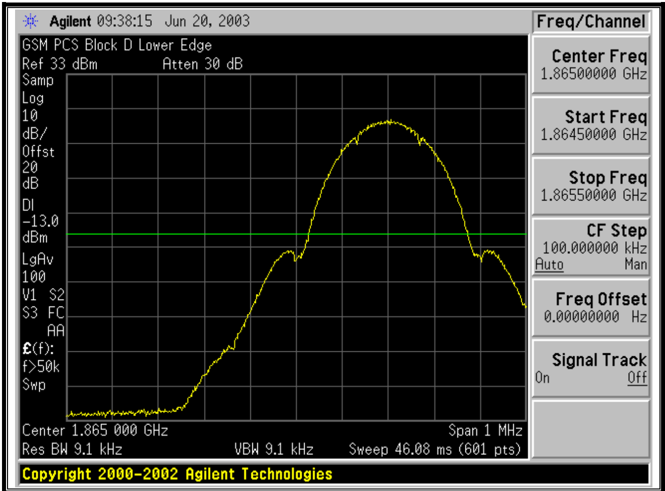
PLOT 11-7: GSM LOWER BAND EDGE D
