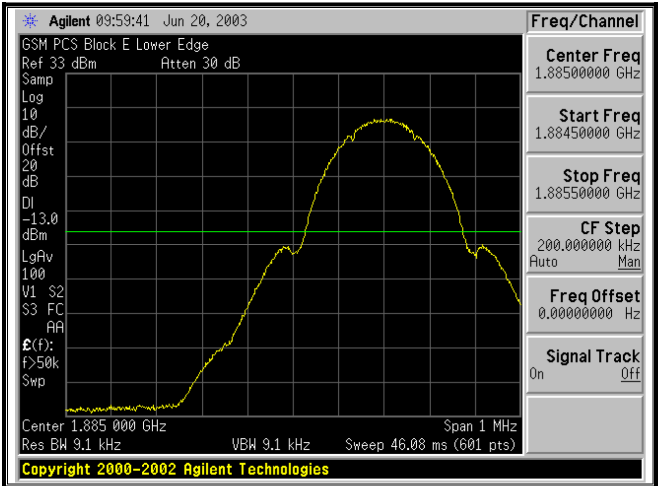
PLOT 11-9: GSM LOWER BAND EDGE E
