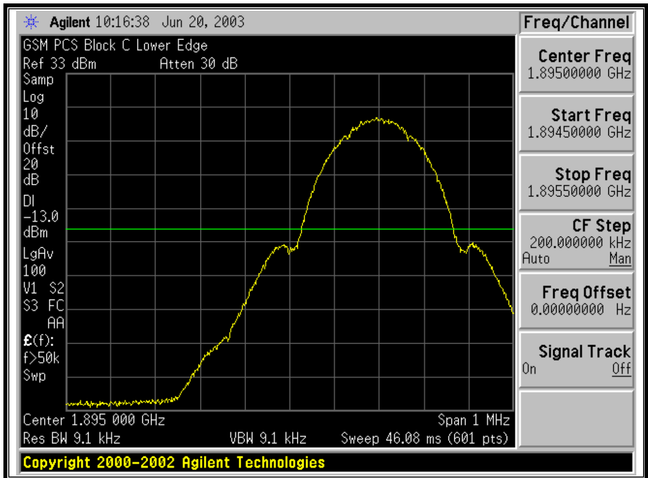
PLOT 11-5: GSM LOWER BAND EDGE C
