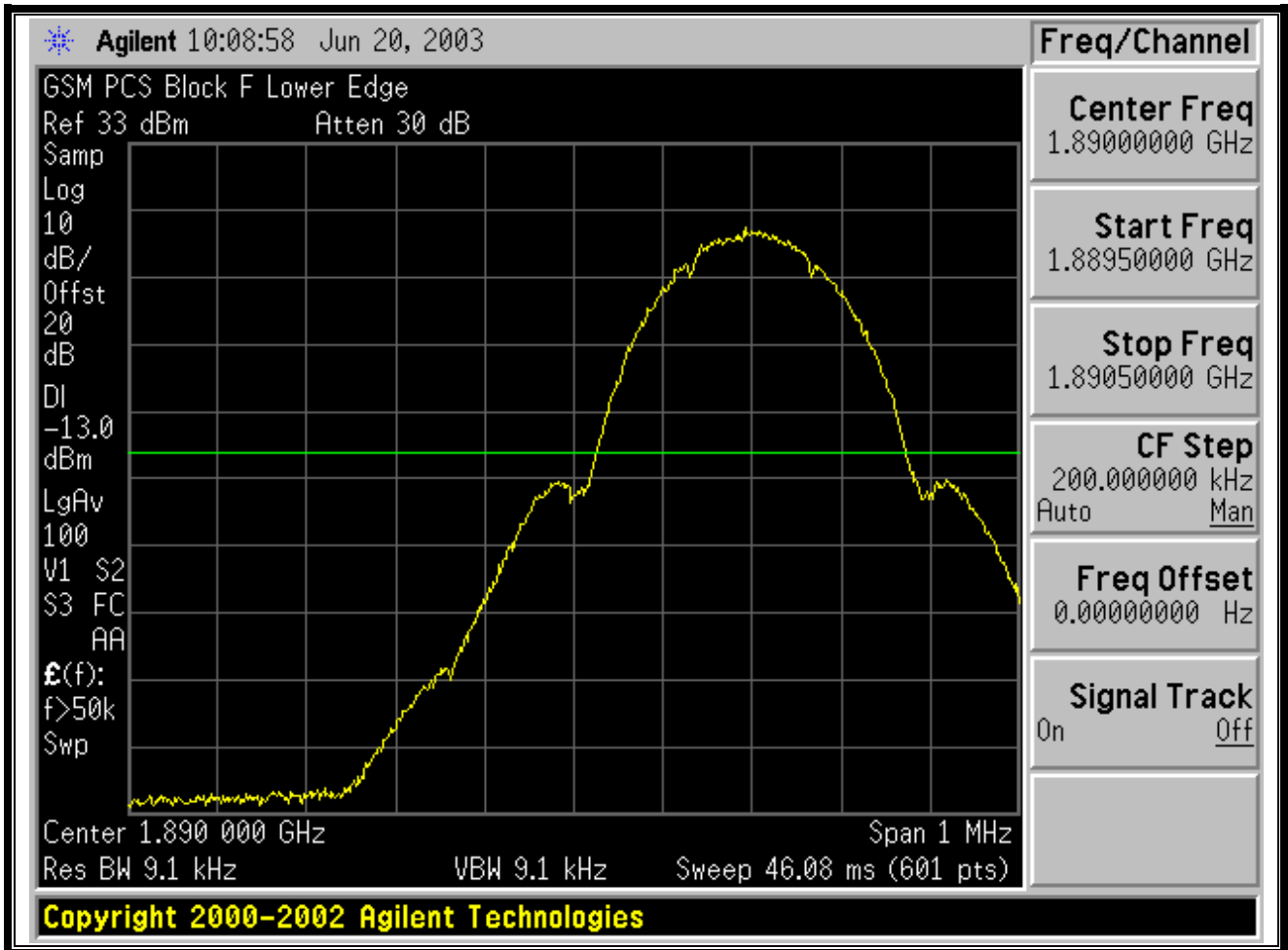
PLOT 11-11: GSM LOWER BAND EDGE F
