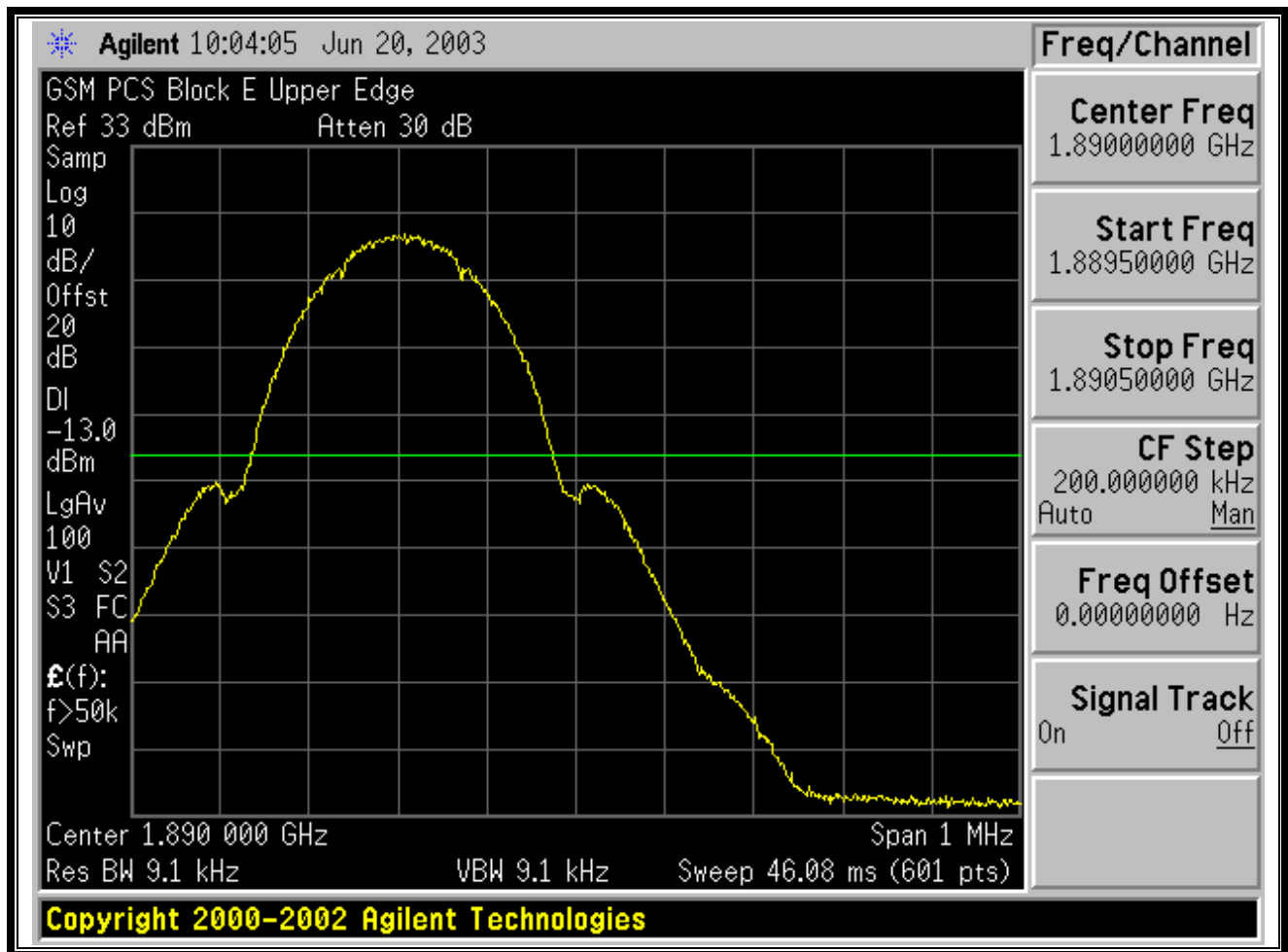
PLOT 11-10: GSM UPPER BAND EDGE E
