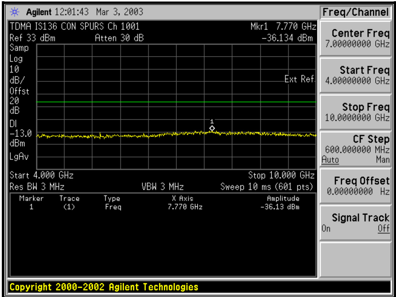
PLOT 9-5: CELLULAR TDMA CONDUCTED SPURIOUS MID CHANNEL
