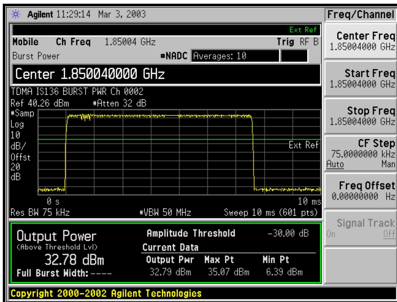
PLOT 4-4: TDMA; BURST POWER; (1850.04 MHZ)
