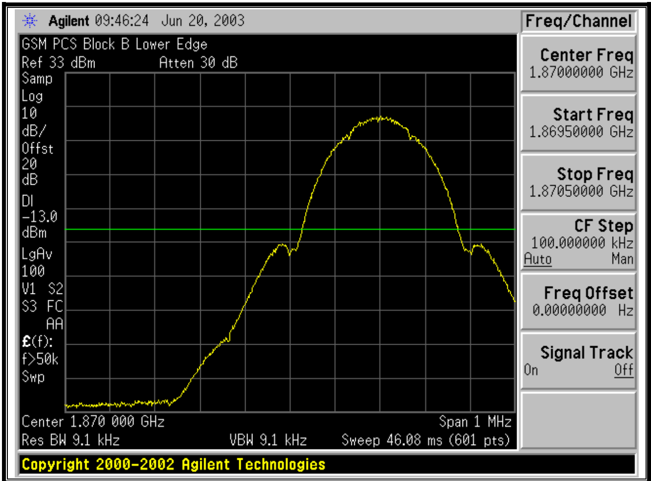
PLOT 11-3: GSM LOWER BAND EDGE B
