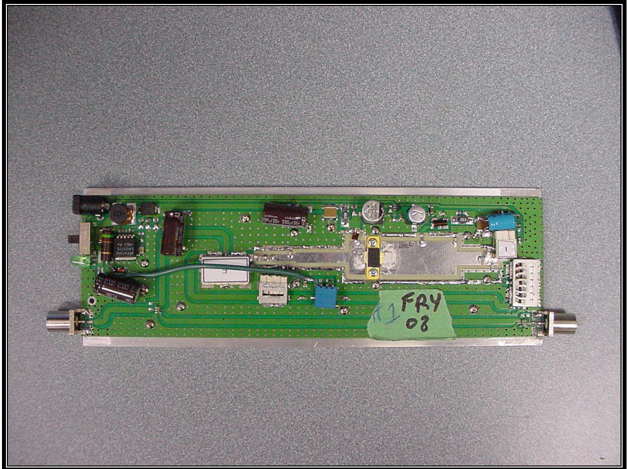
PHOTOGRAPH 12: TOP OF INTERNAL PCB MOUNTED TO HEAT SINK
