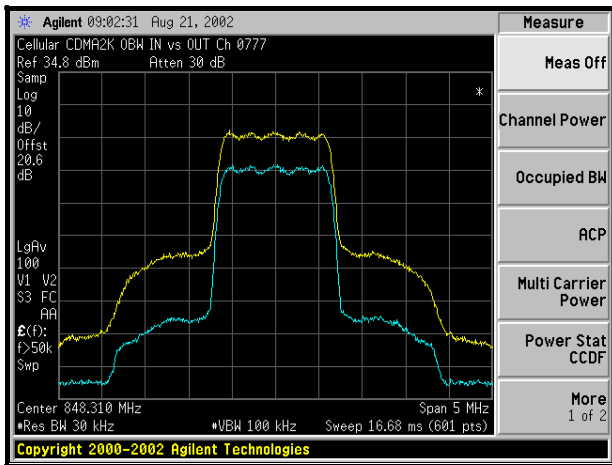
PLOT 6-2: CDMA2000 OBW; IN VS. OUT (CH 777, 848.31 MHZ)
