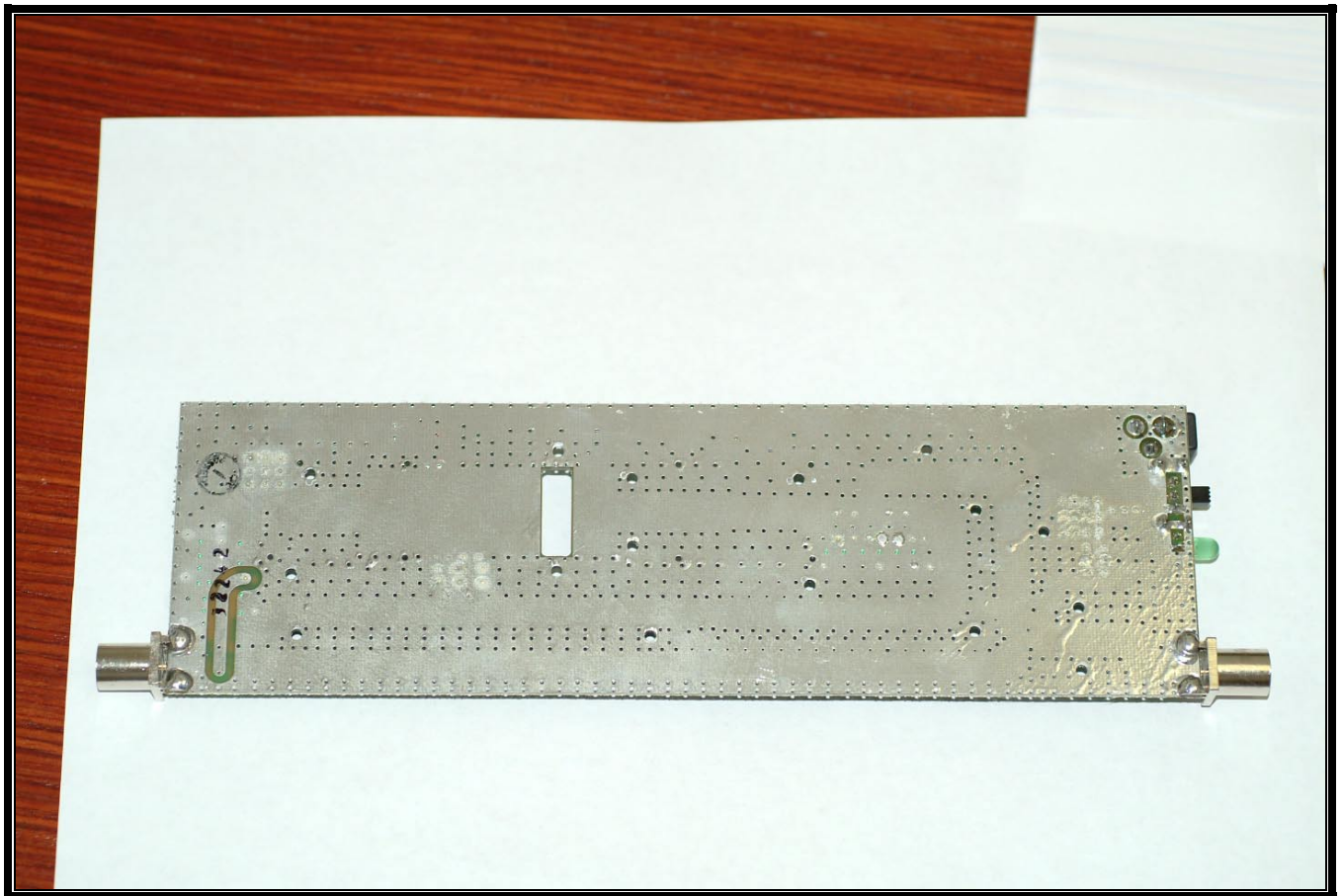
PHOTOGRAPH 14: BOTTOM OF BOARD WITH METAL PLATE REMOVED
