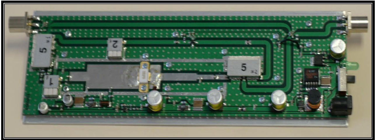
PHOTOGRAPH 12: TOP OF INTERNAL PCB MOUNTED TO HEAT SINK
