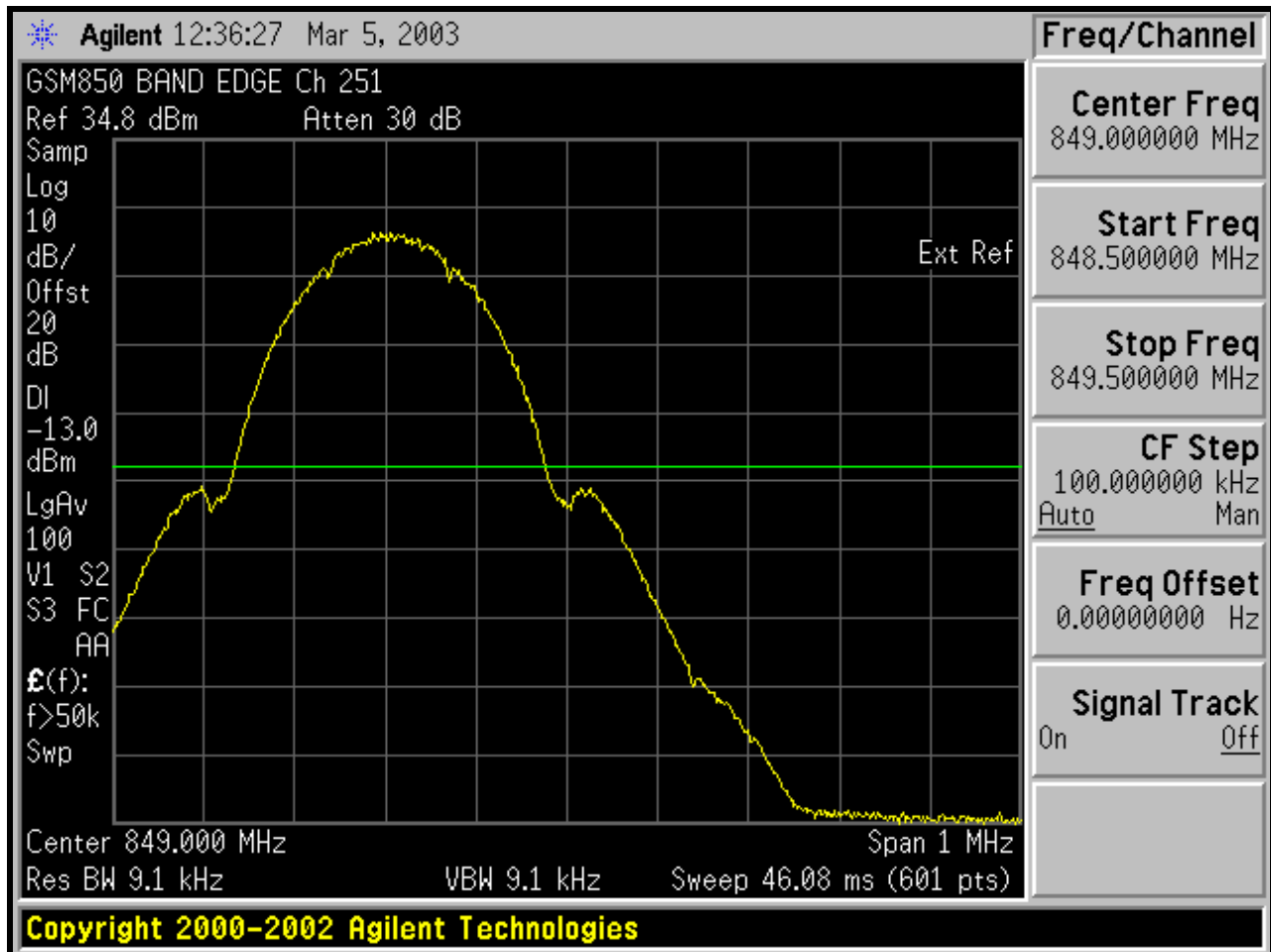
PLOT 11-2: UPPER BAND EDGE D2 849 MHz GSM
