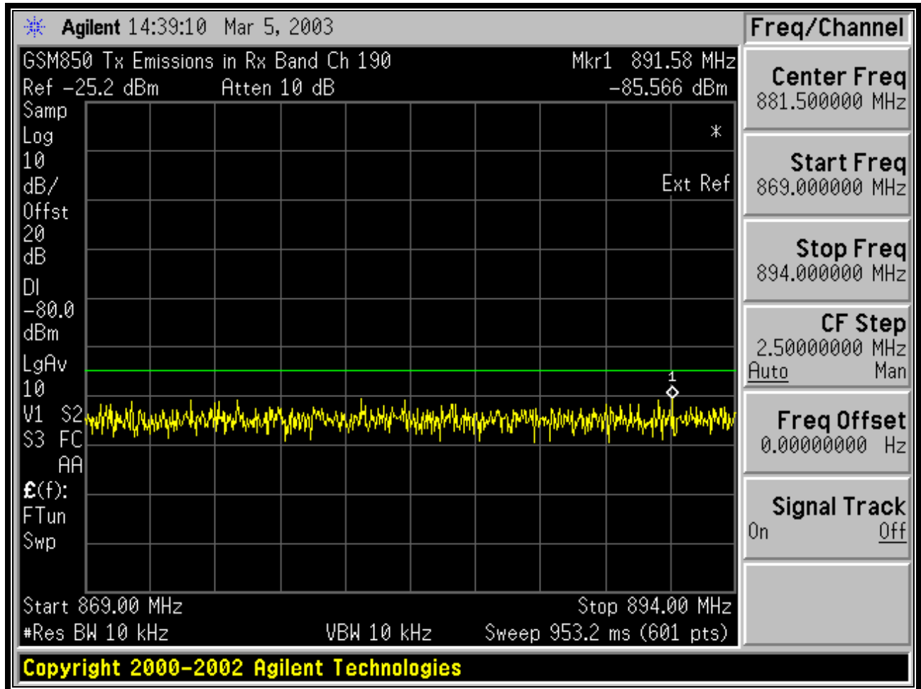
PLOT 12-2: MOBILE EMISSIONS IN BASE STATION BAND; 836.6 MHZ GSM
