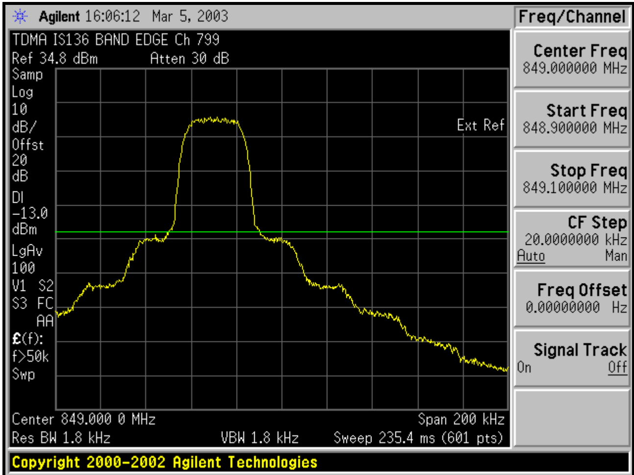
PLOT 11-4 UPPER BAND EDGE A1 849 MHZ TDMA
