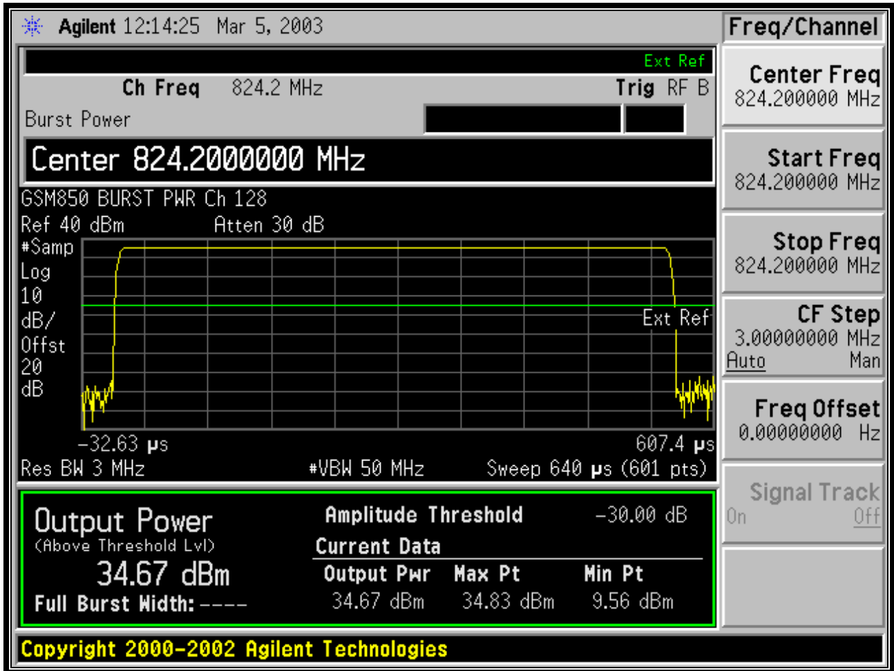
PLOT 4-7: GSM BURST POWER (824.2 MHZ)
