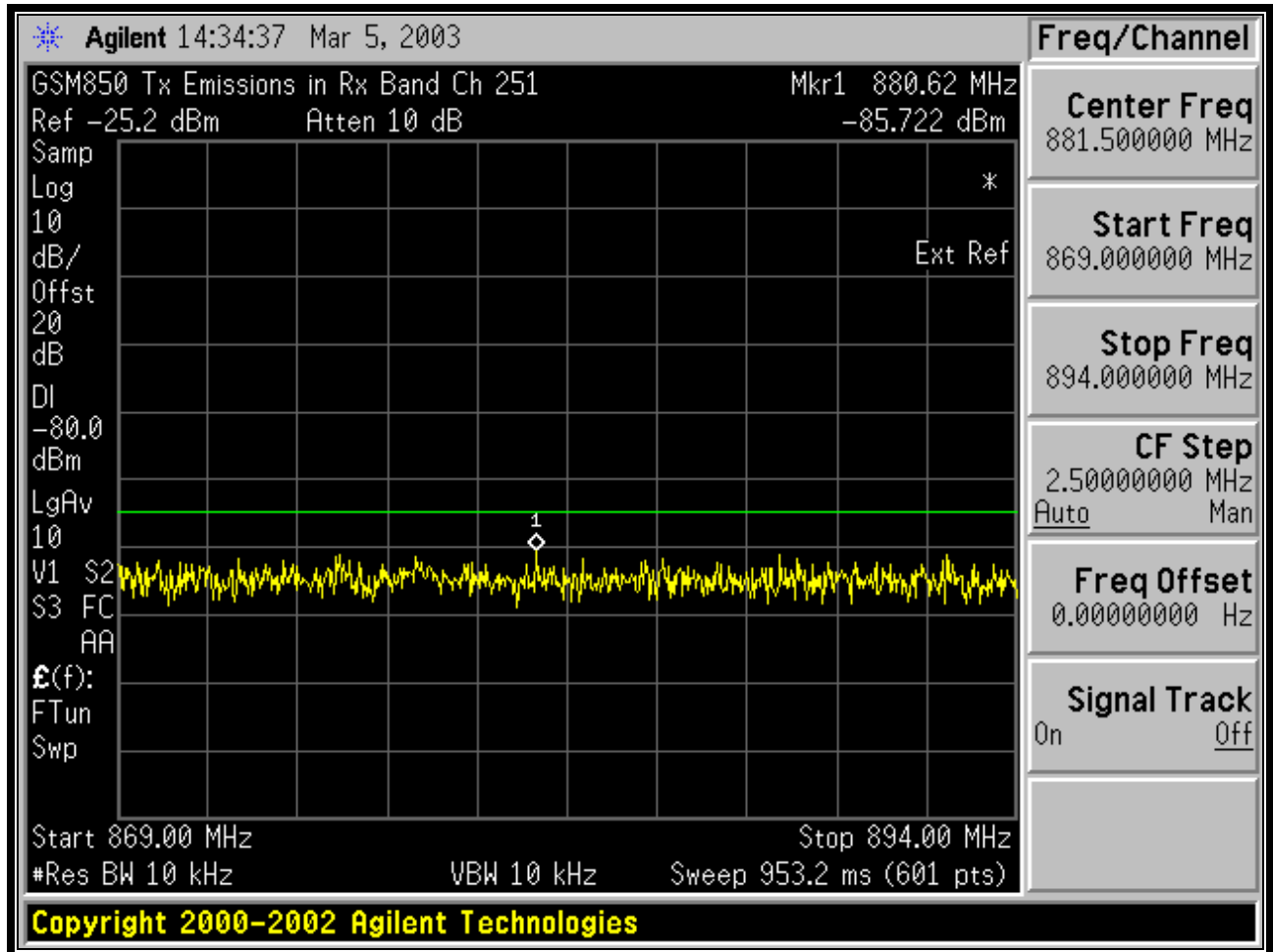
PLOT 12-3: MOBILE EMISSIONS IN BASE STATION BAND; 848.8 MHZ GSM
