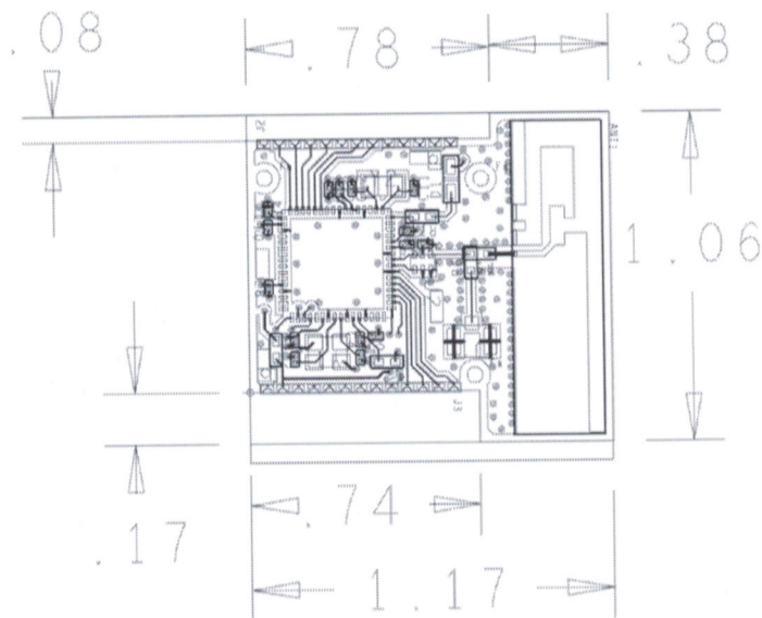
Figure 2: Mechanical dimension of PCB before modification
