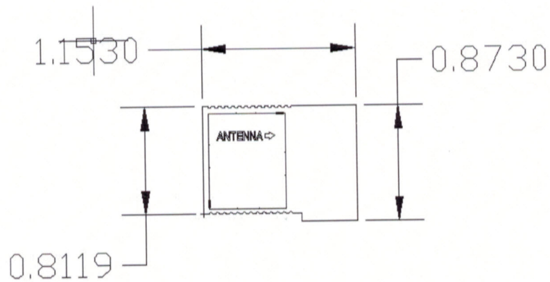
Figure 1: Mechanical dimension of PCB after modification
