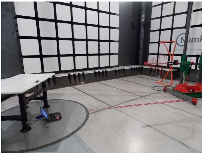
Figure 1.1-1: Field strength setup photo
