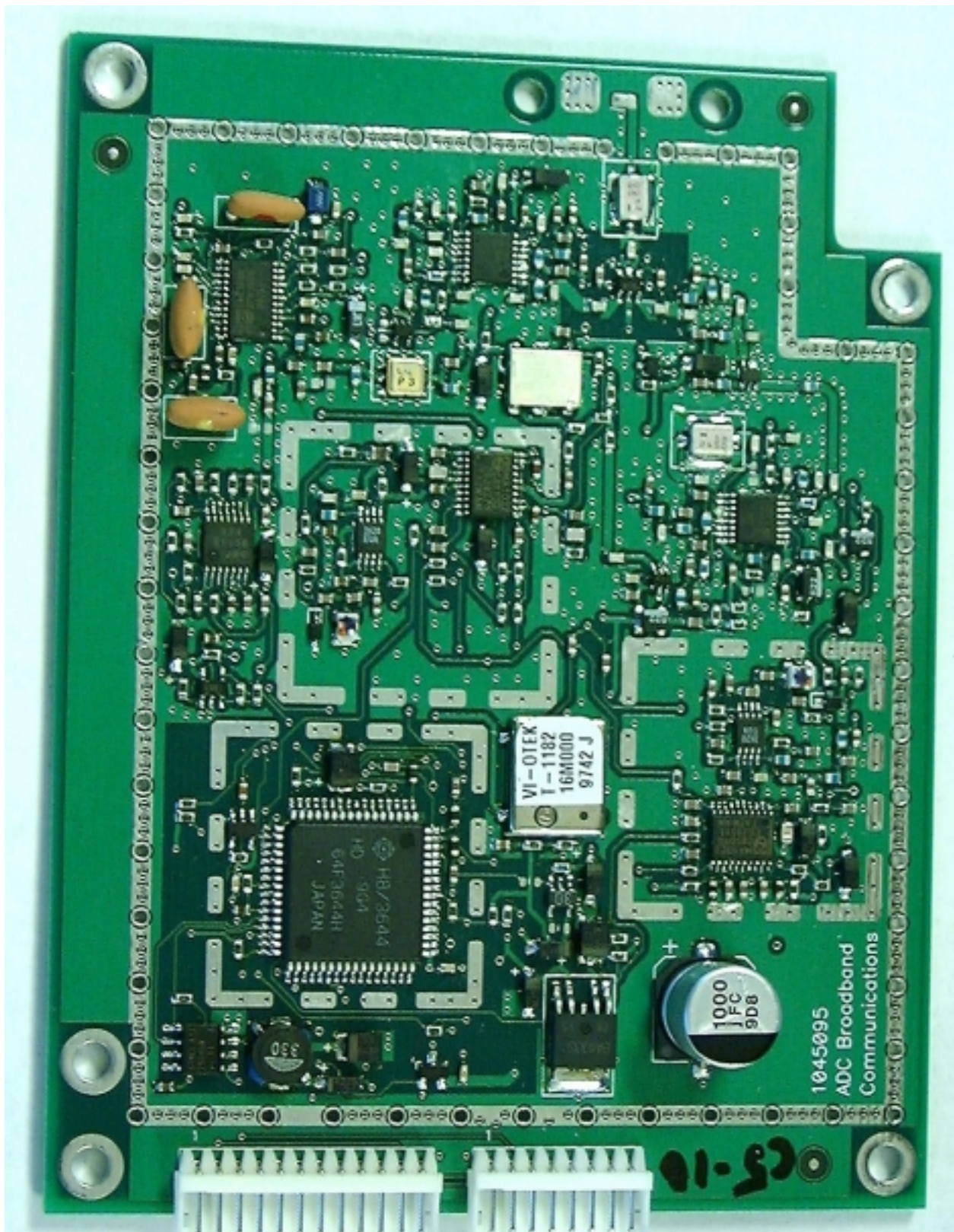
Photo 7. EUT, Top View – Shield and Sub-shields Removed
