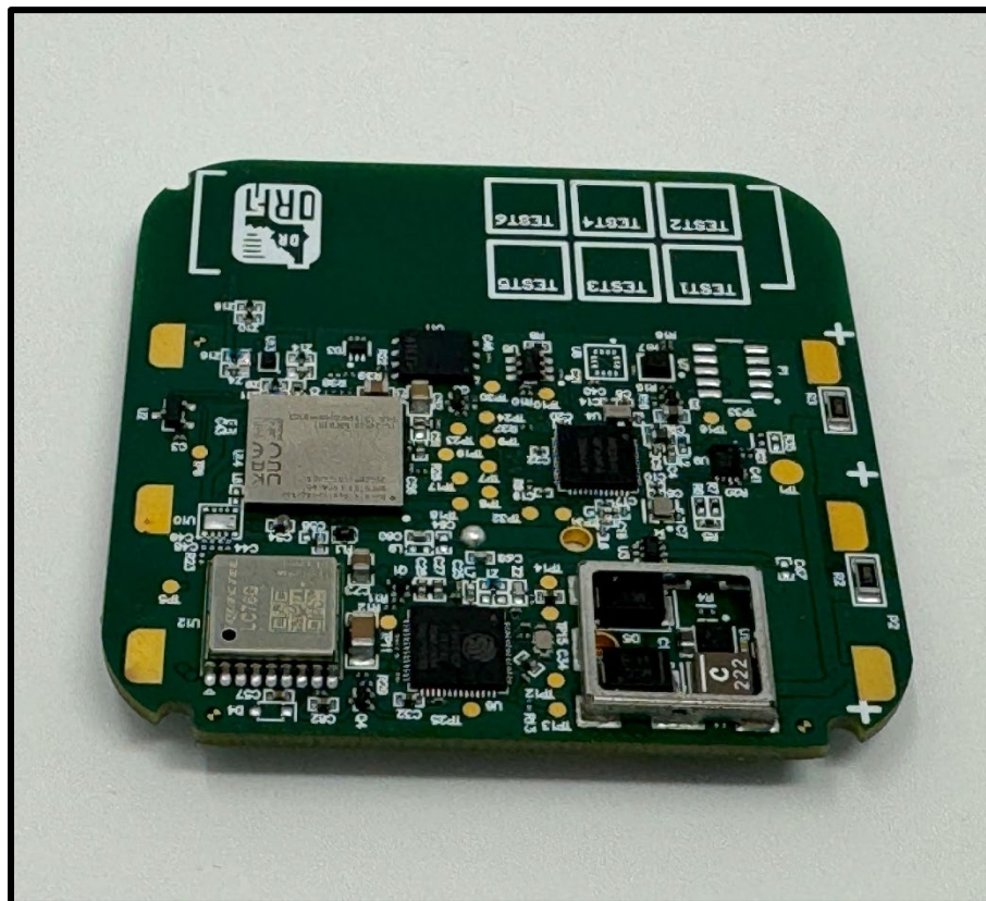
Bottom Orientation 2 – Shield Removed
