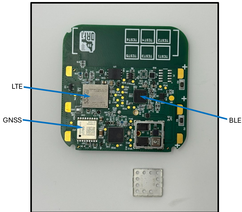
Bottom Orientation 1 – Shield Removed
