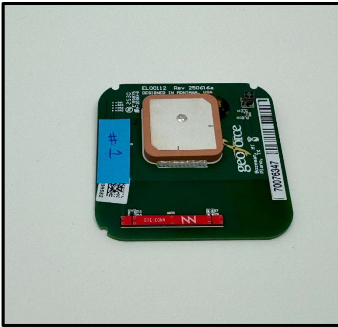
Top Orientation 5
