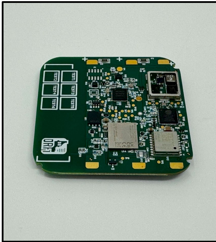
Bottom Orientation 5 – Shield Removed
