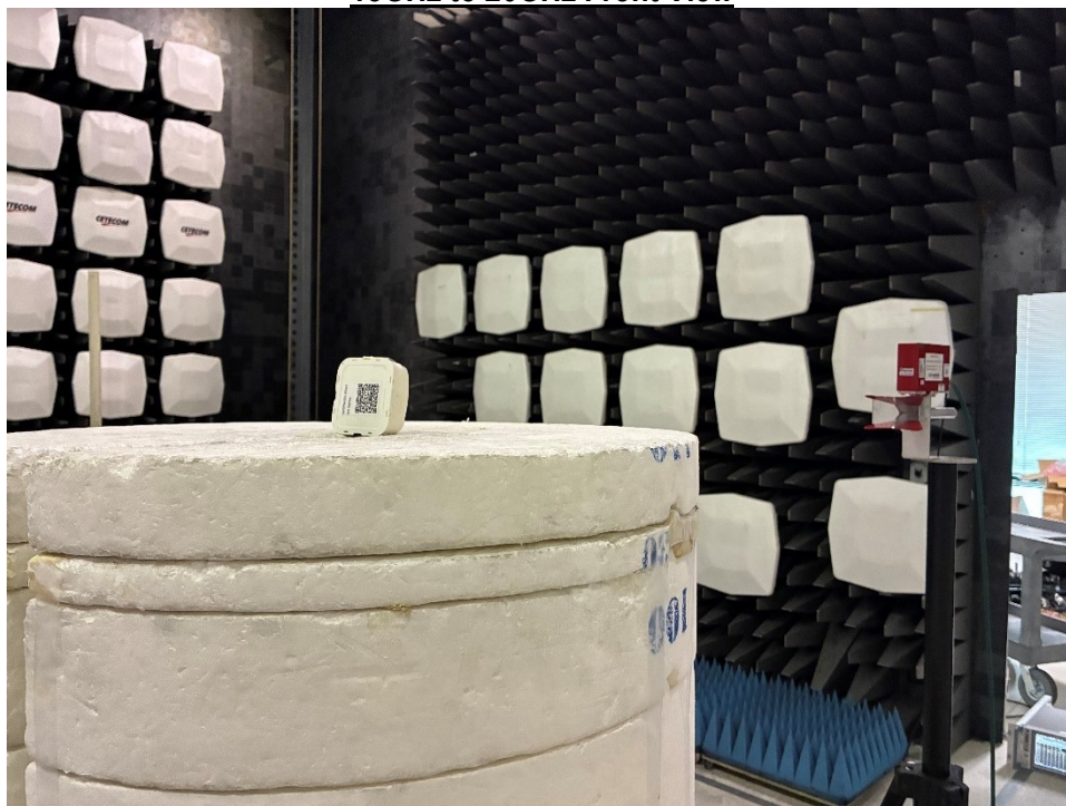
18GHz to 26GHz Front View
