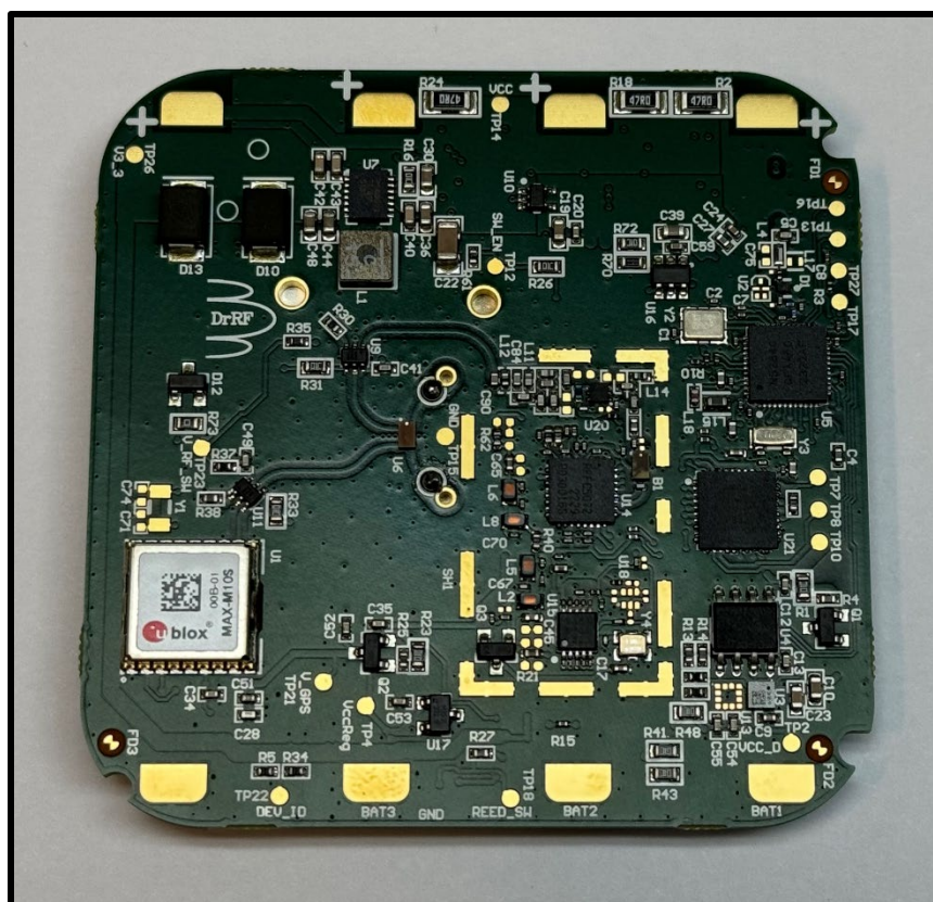
GT0/GT0s PCB Bottom, No Shield Rail
