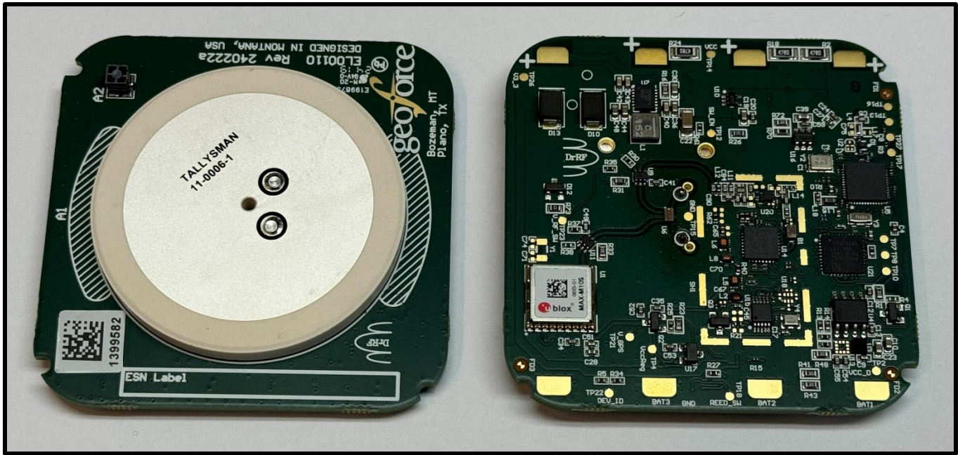
GT1/GT1s General Layout, Top and Bottom
