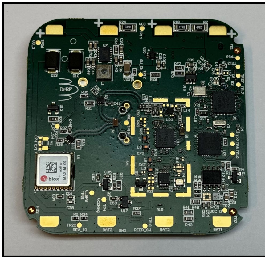
GT1/GT1s PCB Bottom, No Shield Rail
