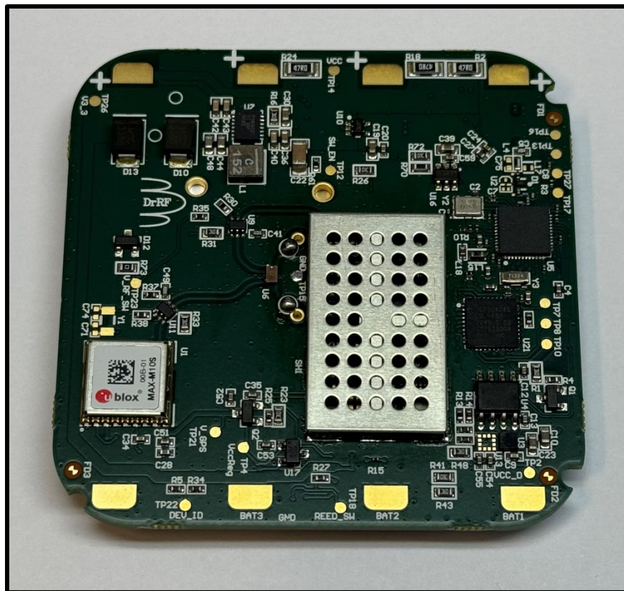
GT1/GT1s PCB Bottom, With Shield Rail and Cover
