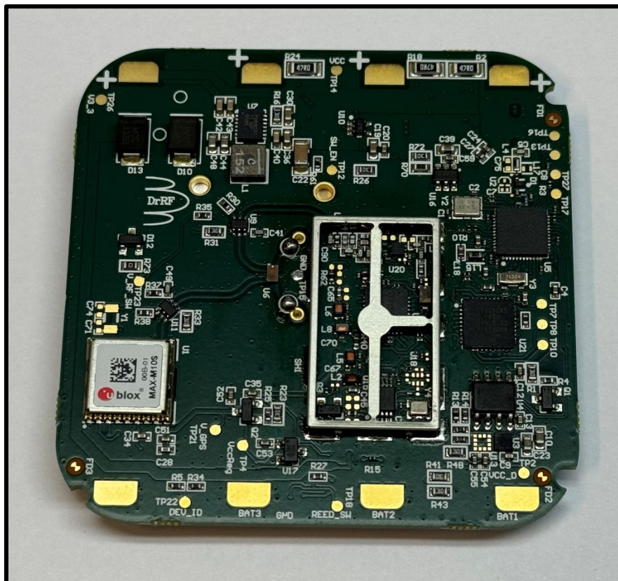
GT0/GT0s PCB Bottom, With Shield Rail
