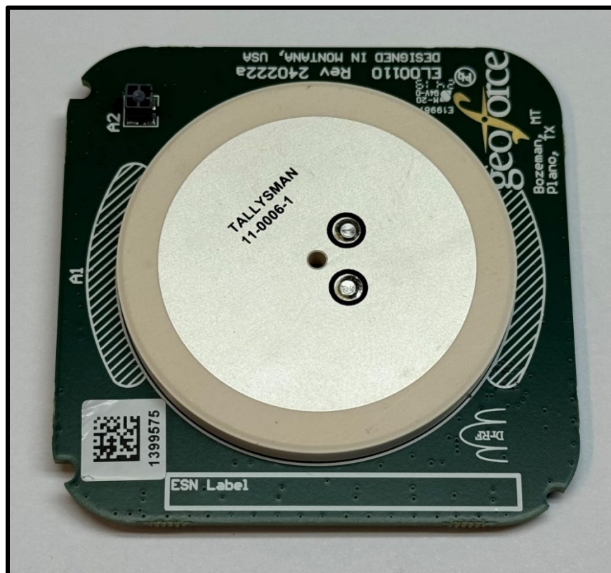
GT0/GT0s PCB Top
