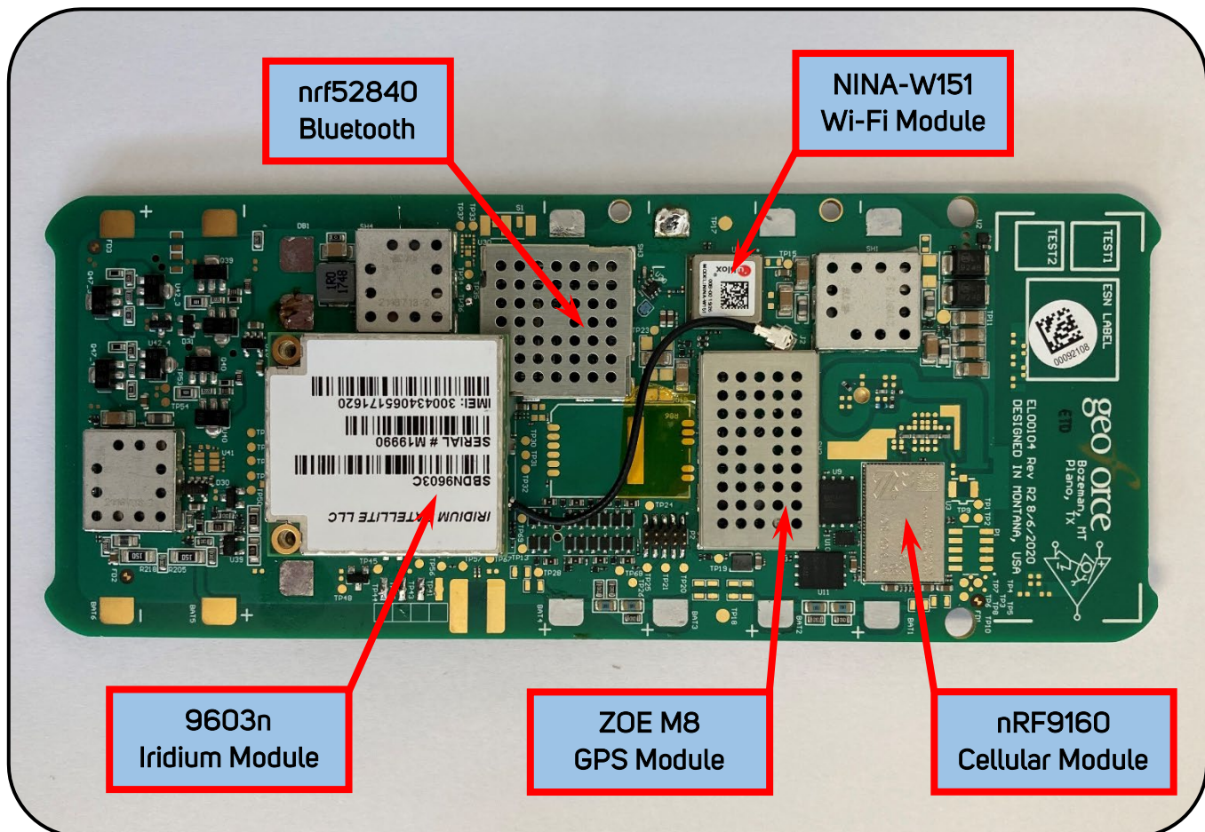
FIGURE 2: COMPONENT SIDE 1
