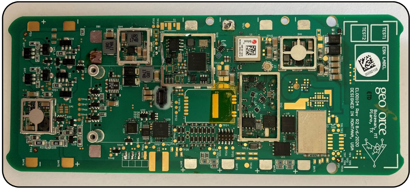
FIGURE 3: COMPONENT SIDE WITHOUT SHIELDS
