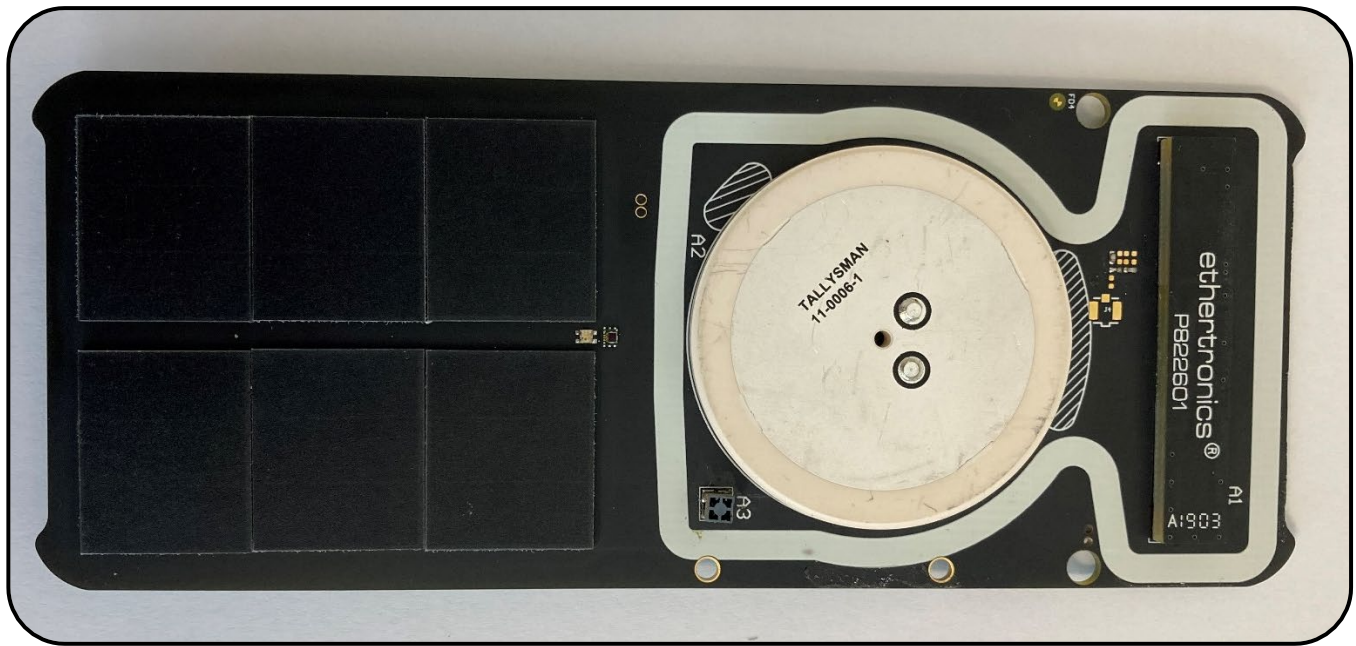
FIGURE 1: ANTENNA SIDE
