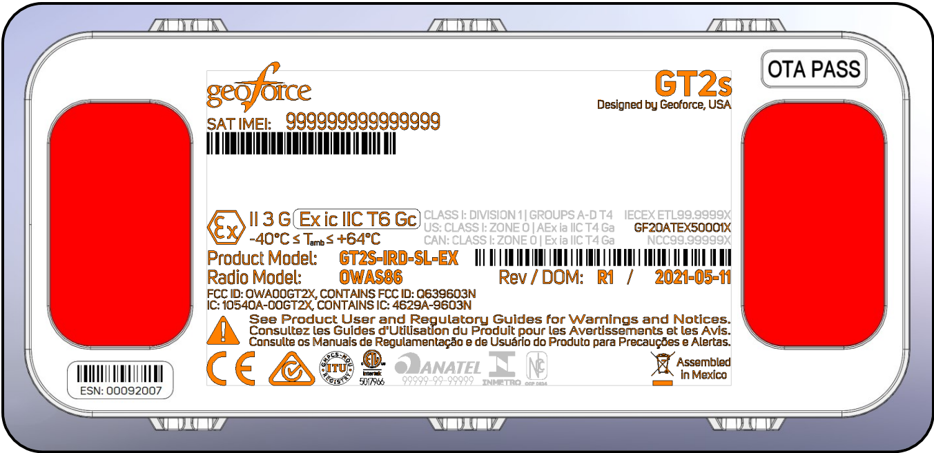
FIGURE 4: GT2s BOTTOM SIDE
