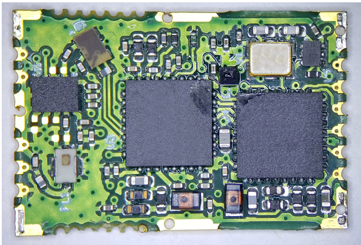
Figure 1. Radio Module, Top, without Shield
