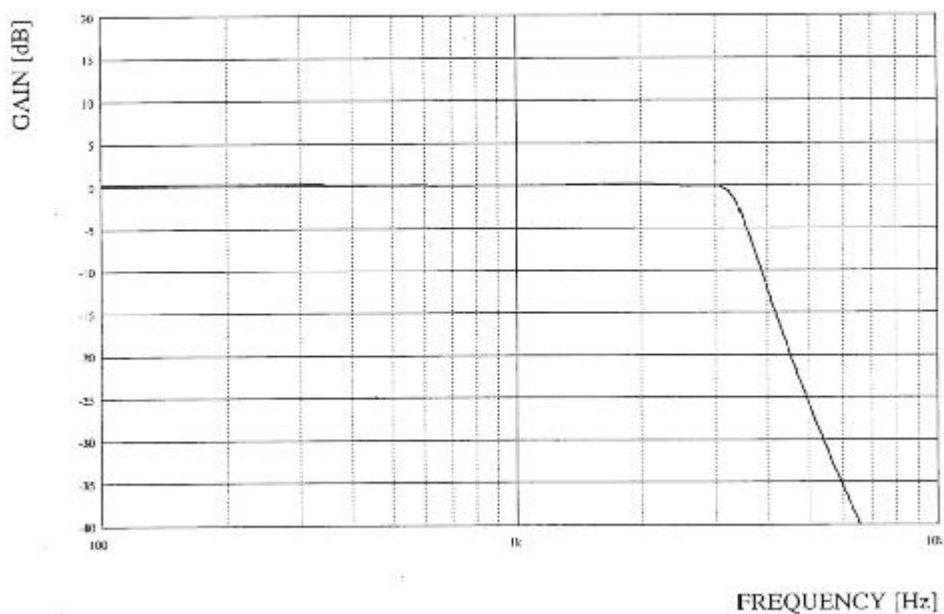
Fig 4.A LPF( F_c=3.0\text{kHz} ) Frequency Response (Reference)
