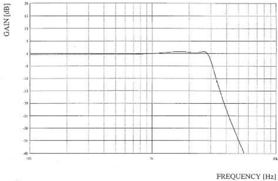
Fig.4 B LPF( F_c=2.55\text{kHz} ) Frequency Response (Reference)
