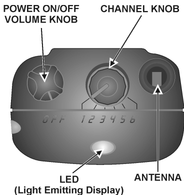
Figure 1 – PANTHER 300P Radio Top View
