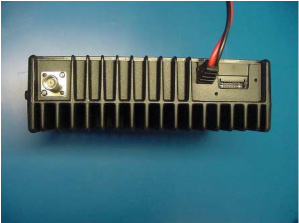
PHOTOGRAPH 15: REAR VIEW
