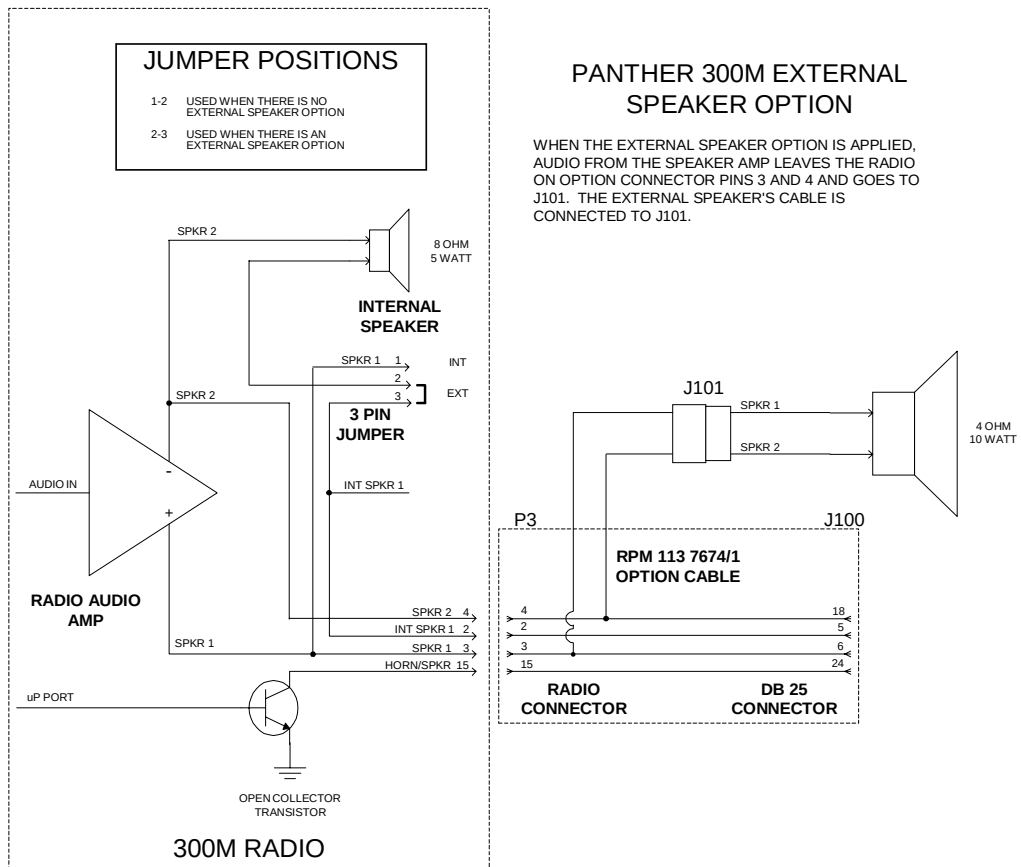
Figure 11 – External Speaker Option
