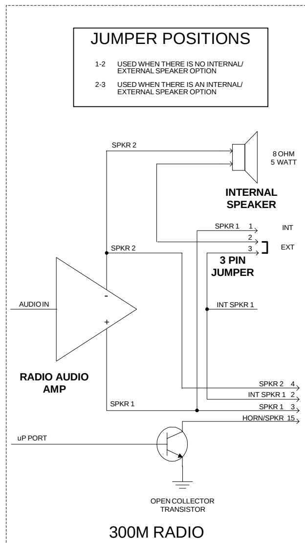
Figure 12 – Internal/External Speaker Relay
