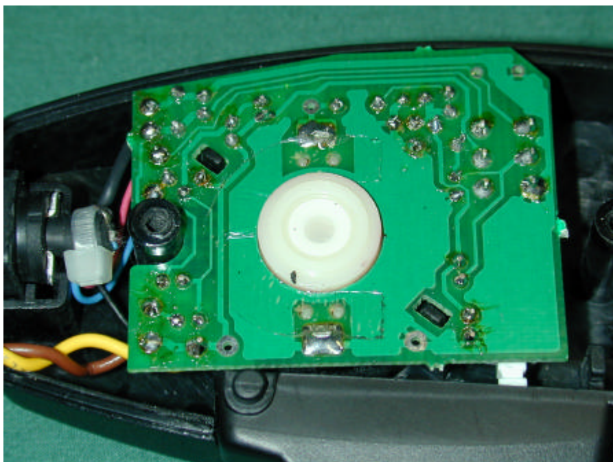
Internal mic/speaker solder side
