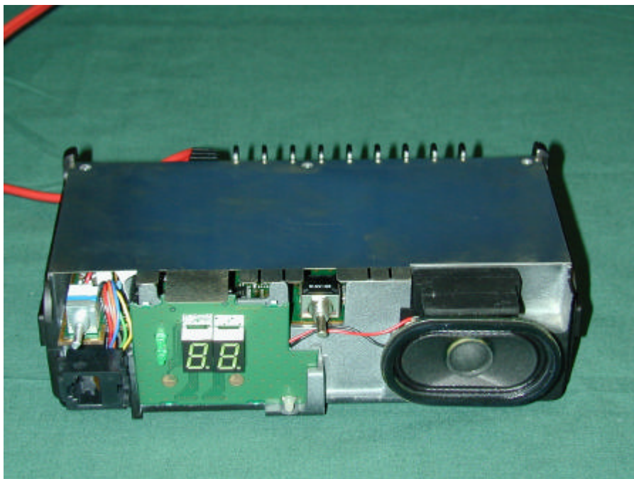
Internal front view
