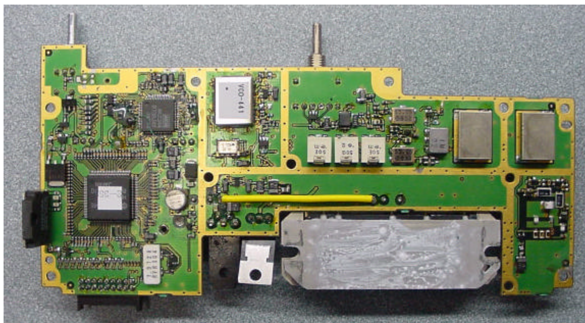
PCB Side B
