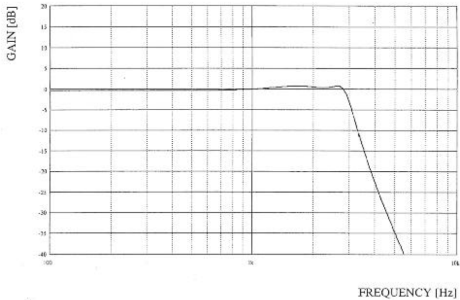
Fig.4 B LPF( F_c=2.35\text{kHz} ) Frequency Response (Reference)
