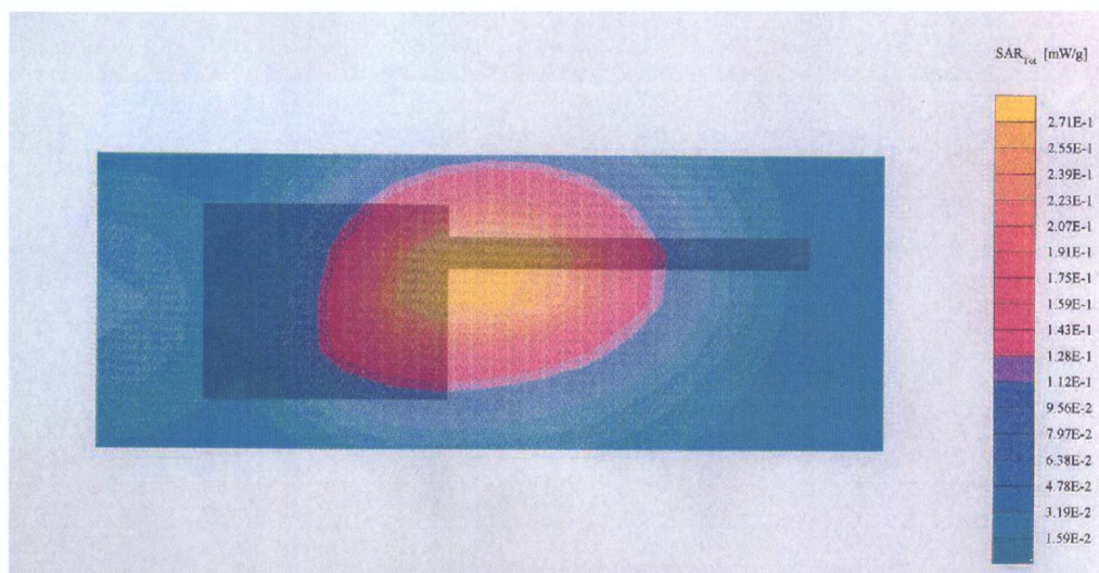
Configuration 6, clip touching
