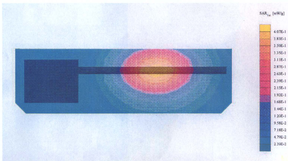
Configuration 5, clip touching
